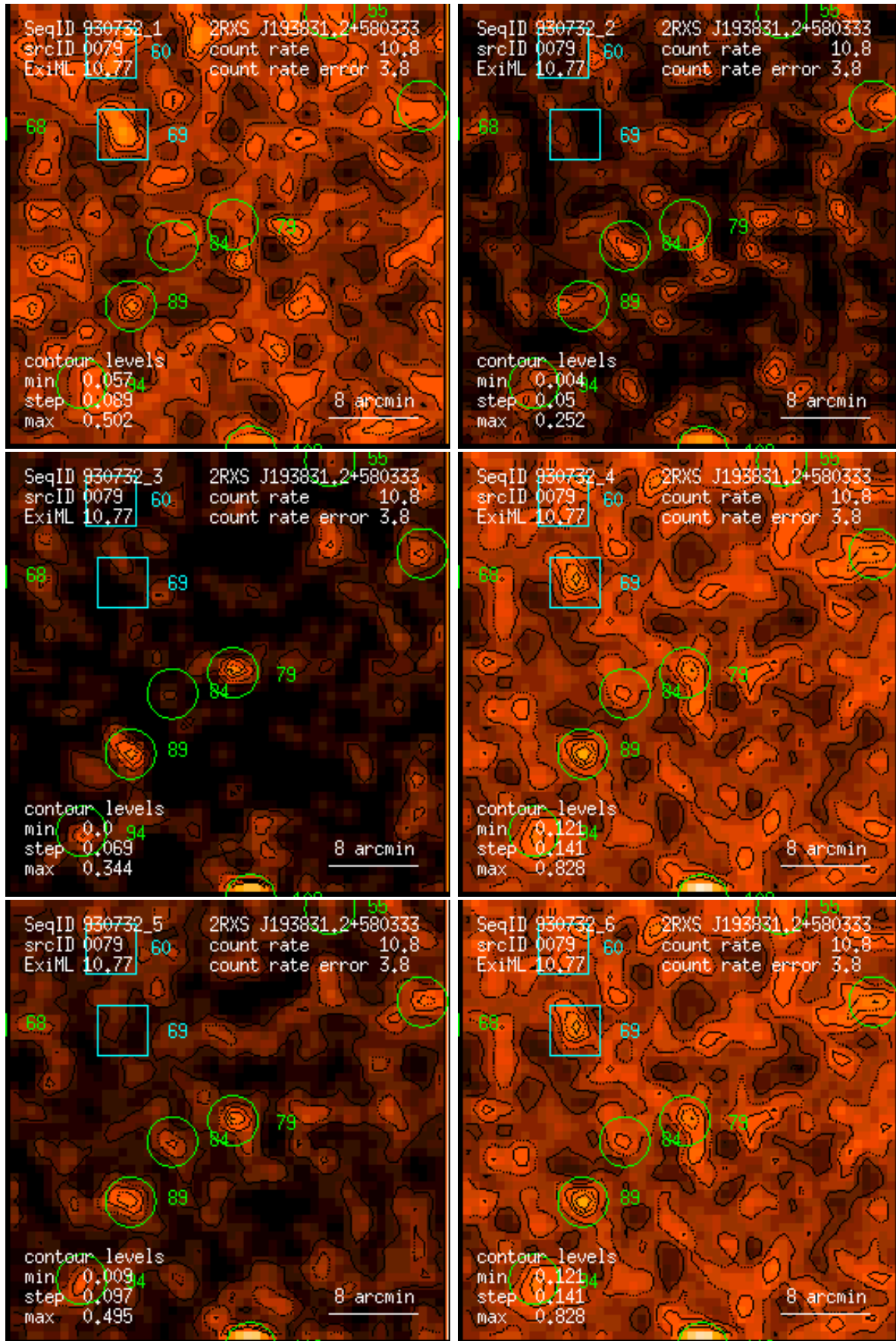
Figure 79: RASS 930732: detection 0079: band rate images, Gaussian filter: (1) PSPC channels 11 – 41, (2) 52 – 90, (3) 91 – 201, (4) 11 – 235, (5) 52 – 201, (6) 11 – 201. Broad band rates in counts/ks. Band rate contour levels in counts/ks/arcmin 2 .
