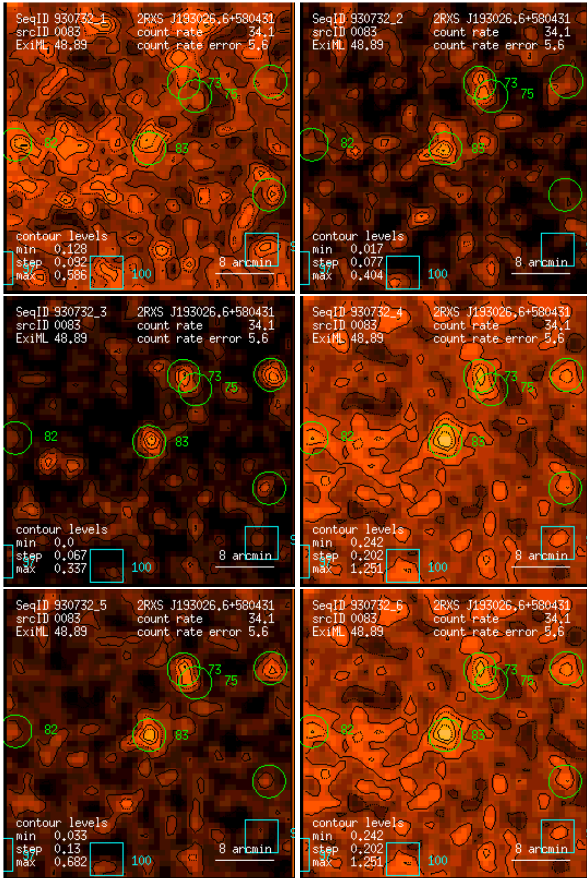
Figure 83: RASS 930732: detection 0083: band rate images, Gaussian filter: (1) PSPC channels 11 – 41, (2) 52 – 90, (3) 91 – 201, (4) 11 – 235, (5) 52 – 201, (6) 11 – 201. Broad band rates in counts/ks. Band rate contour levels in counts/ks/arcmin 2 .
