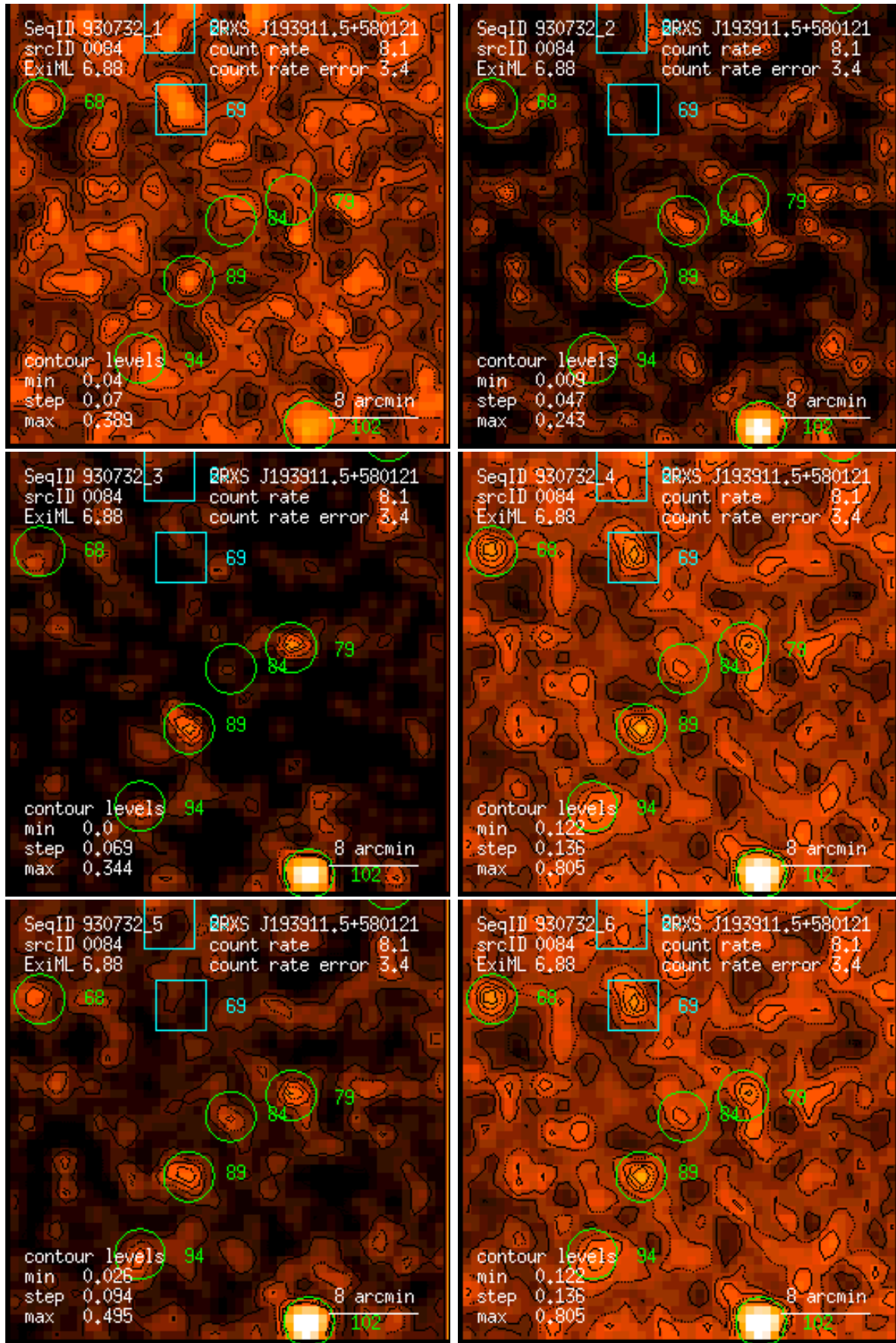
Figure 84: RASS 930732: detection 0084: band rate images, Gaussian filter: (1) PSPC channels 11 – 41, (2) 52 – 90, (3) 91 – 201, (4) 11 – 235, (5) 52 – 201, (6) 11 – 201. Broad band rates in counts/ks. Band rate contour levels in counts/ks/arcmin 2 .
