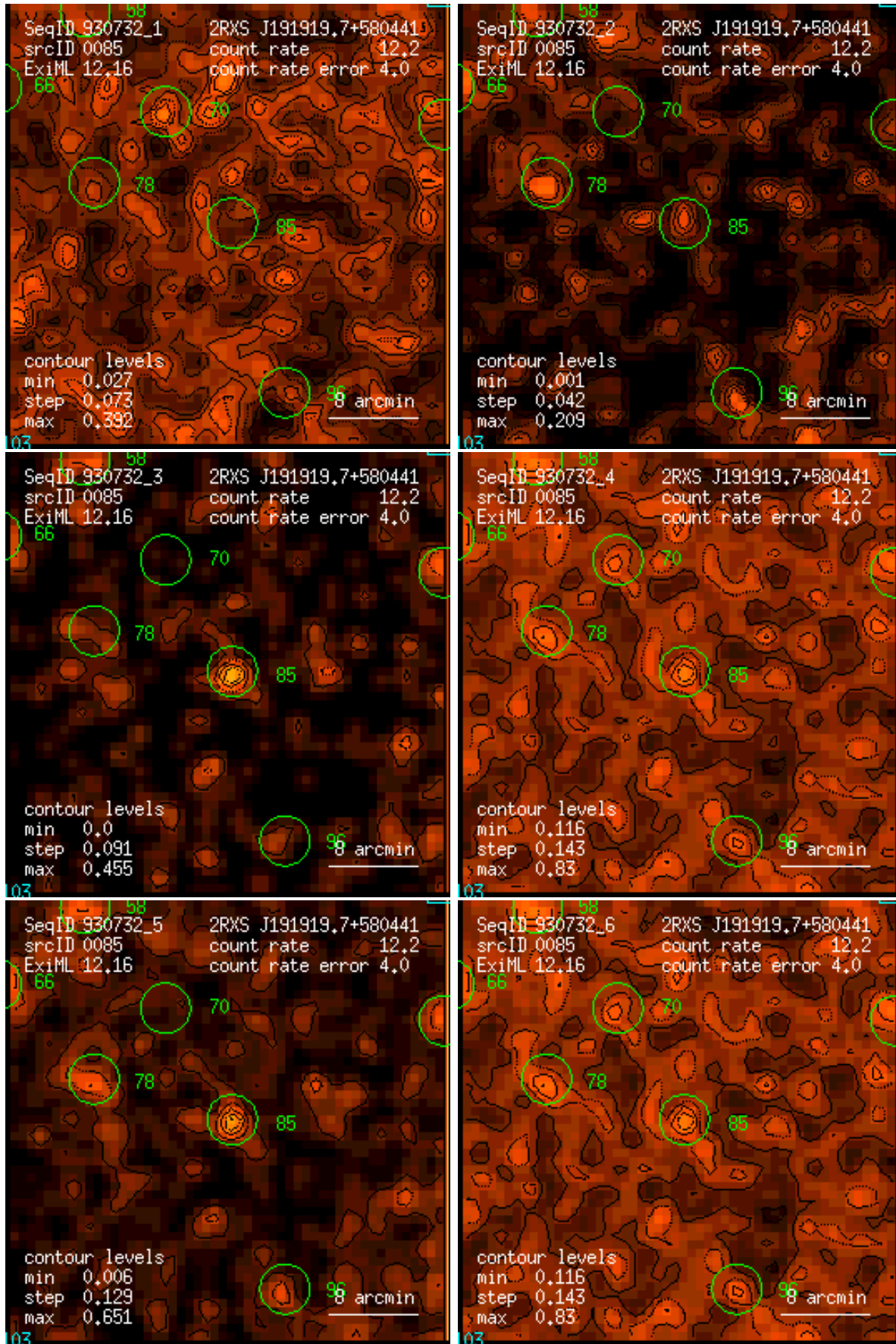
Figure 85: RASS 930732: detection 0085: band rate images, Gaussian filter: (1) PSPC channels 11 – 41, (2) 52 – 90, (3) 91 – 201, (4) 11 – 235, (5) 52 – 201, (6) 11 – 201. Broad band rates in counts/ks. Band rate contour levels in counts/ks/arcmin 2 .
