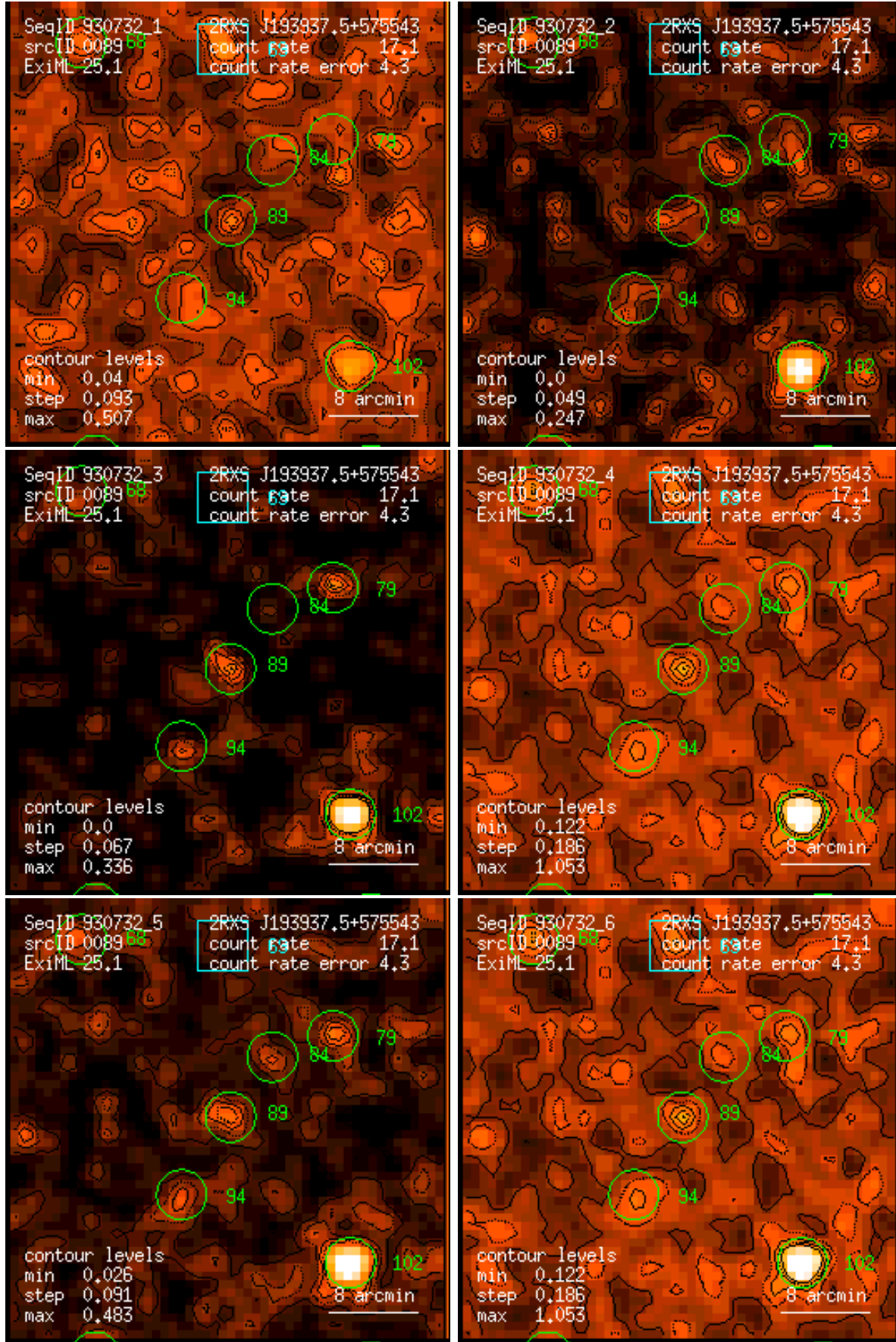
Figure 89: RASS 930732: detection 0089: band rate images, Gaussian filter: (1) PSPC channels 11 – 41, (2) 52 – 90, (3) 91 – 201, (4) 11 – 235, (5) 52 – 201, (6) 11 – 201. Broad band rates in counts/ks. Band rate contour levels in counts/ks/arcmin 2 .
