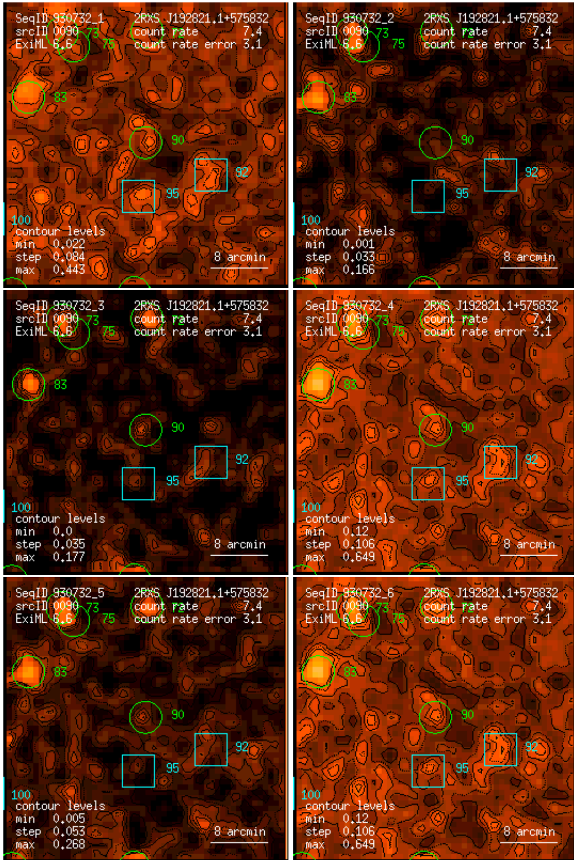
Figure 90: RASS 930732: detection 0090: band rate images, Gaussian filter: (1) PSPC channels 11 – 41, (2) 52 – 90, (3) 91 – 201, (4) 11 – 235, (5) 52 – 201, (6) 11 – 201. Broad band rates in counts/ks. Band rate contour levels in counts/ks/arcmin 2 .
