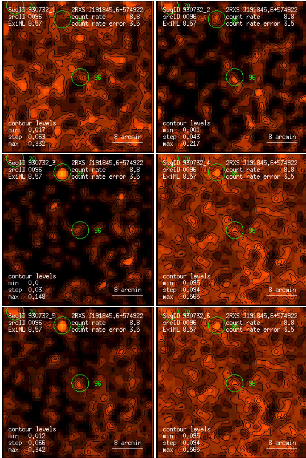
Figure 96: RASS 930732: detection 0096: band rate images, Gaussian filter: (1) PSPC channels 11 – 41, (2) 52 – 90, (3) 91 – 201, (4) 11 – 235, (5) 52 – 201, (6) 11 – 201. Broad band rates in counts/ks. Band rate contour levels in counts/ks/arcmin 2 .
