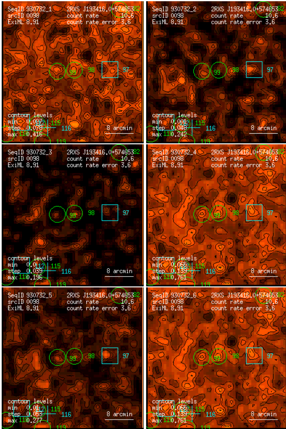
Figure 98: RASS 930732: detection 0098: band rate images, Gaussian filter: (1) PSPC channels 11 – 41, (2) 52 – 90, (3) 91 – 201, (4) 11 – 235, (5) 52 – 201, (6) 11 – 201. Broad band rates in counts/ks. Band rate contour levels in counts/ks/arcmin 2 .
