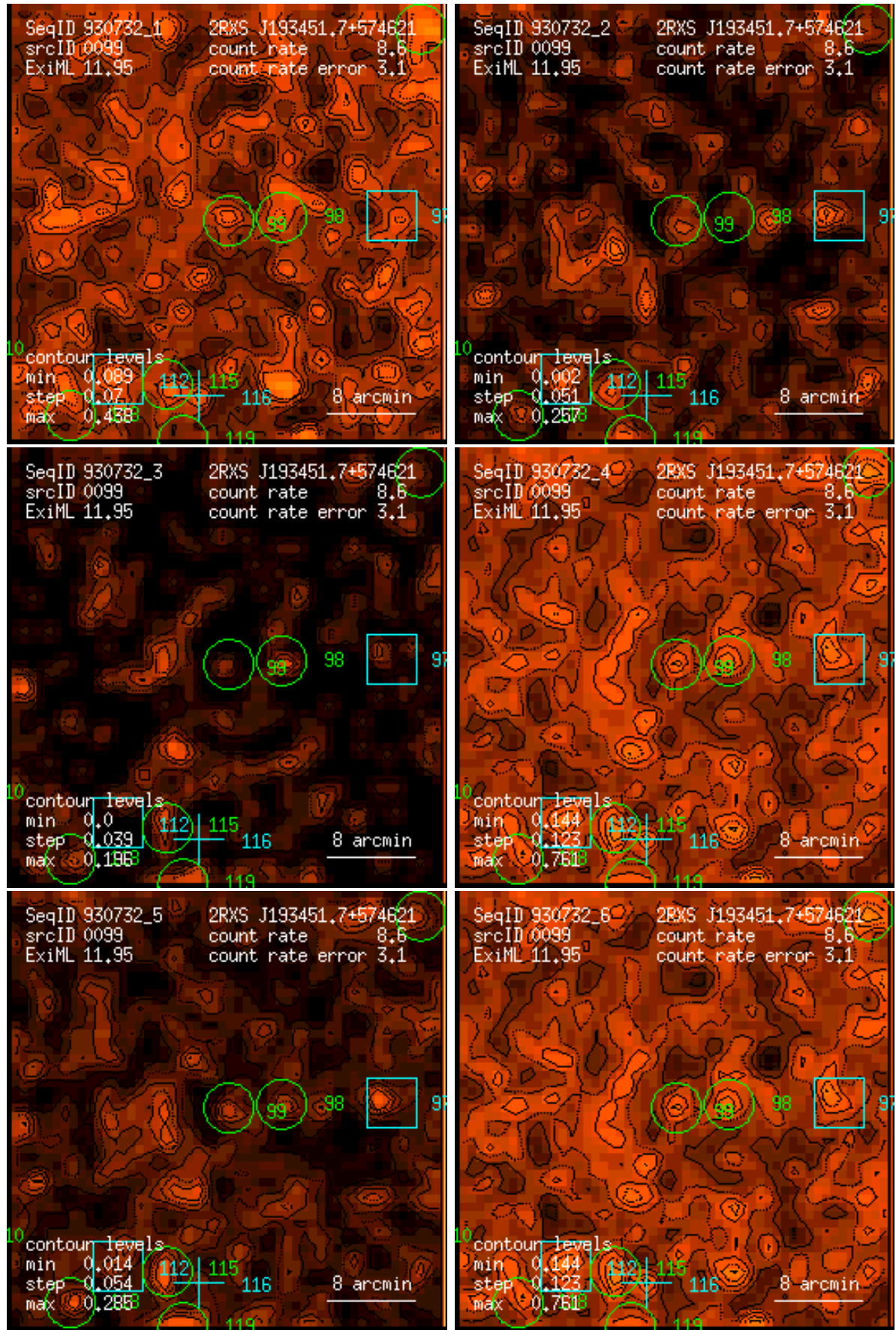
Figure 99: RASS 930732: detection 0099: band rate images, Gaussian filter: (1) PSPC channels 11 – 41, (2) 52 – 90, (3) 91 – 201, (4) 11 – 235, (5) 52 – 201, (6) 11 – 201. Broad band rates in counts/ks. Band rate contour levels in counts/ks/arcmin 2 .
