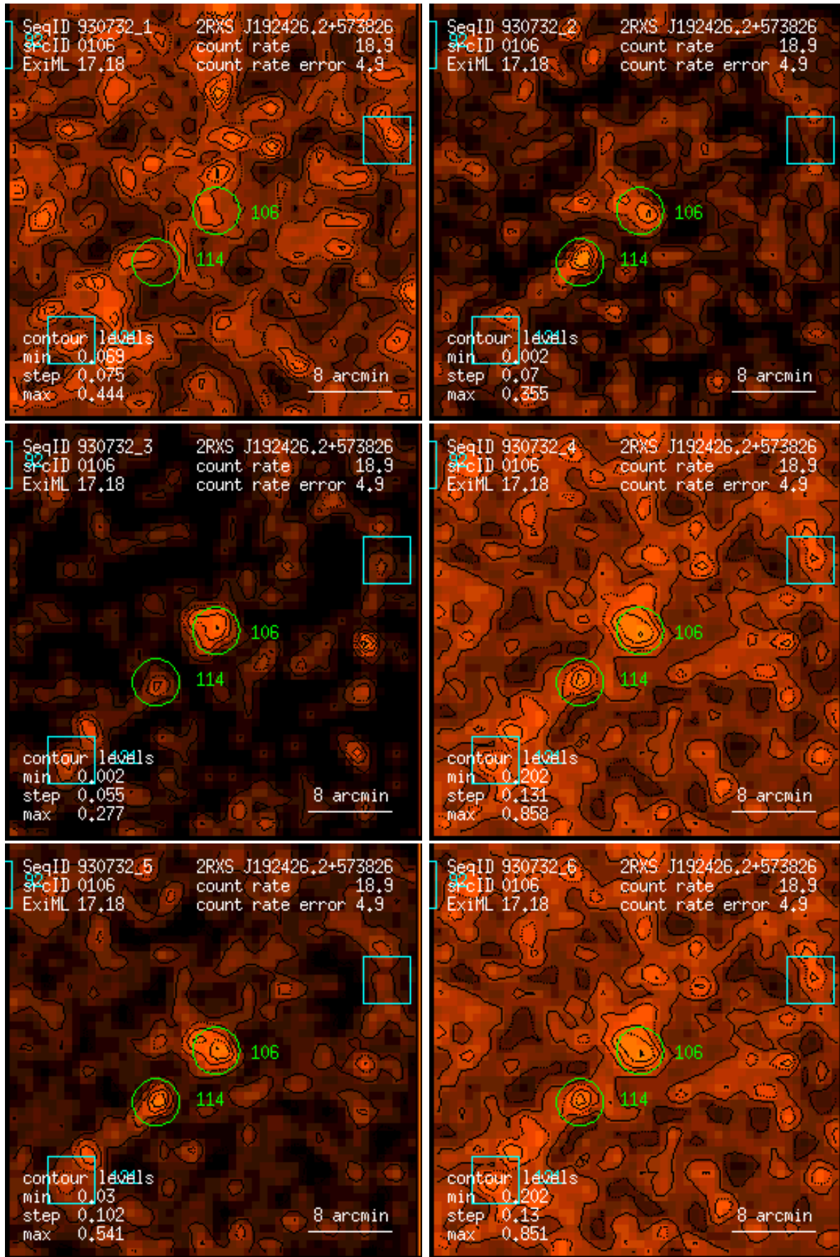
Figure 106: RASS 930732: detection 0106: band rate images, Gaussian filter: (1) PSPC channels 11 – 41, (2) 52 – 90, (3) 91 – 201, (4) 11 – 235, (5) 52 – 201, (6) 11 – 201. Broad band rates in counts/ks. Band rate contour levels in counts/ks/arcmin 2 .
