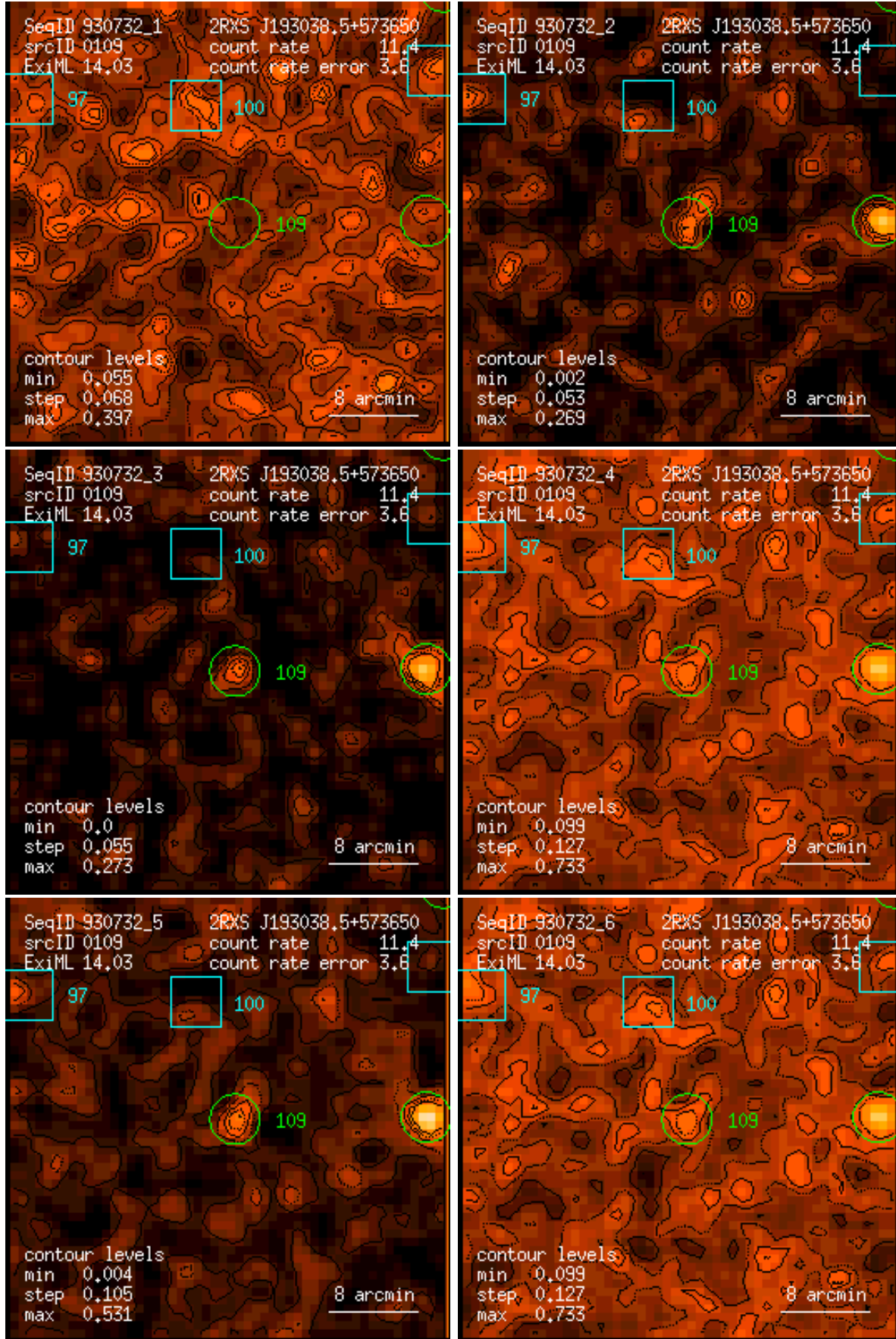
Figure 109: RASS 930732: detection 0109: band rate images, Gaussian filter: (1) PSPC channels 11 – 41, (2) 52 – 90, (3) 91 – 201, (4) 11 – 235, (5) 52 – 201, (6) 11 – 201. Broad band rates in counts/ks. Band rate contour levels in counts/ks/arcmin 2 .
