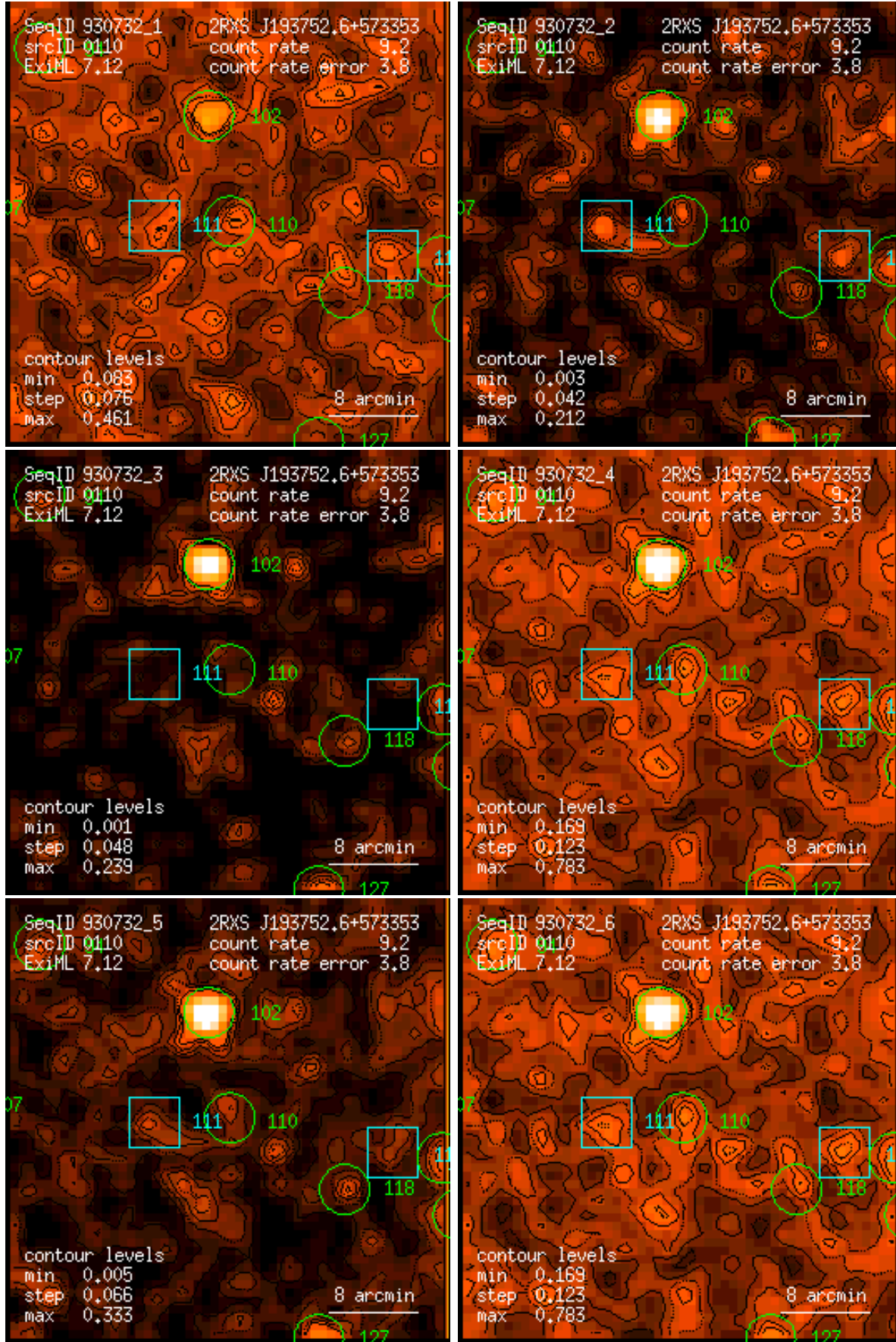
Figure 110: RASS 930732: detection 0110: band rate images, Gaussian filter: (1) PSPC channels 11 – 41, (2) 52 – 90, (3) 91 – 201, (4) 11 – 235, (5) 52 – 201, (6) 11 – 201. Broad band rates in counts/ks. Band rate contour levels in counts/ks/arcmin 2 .
