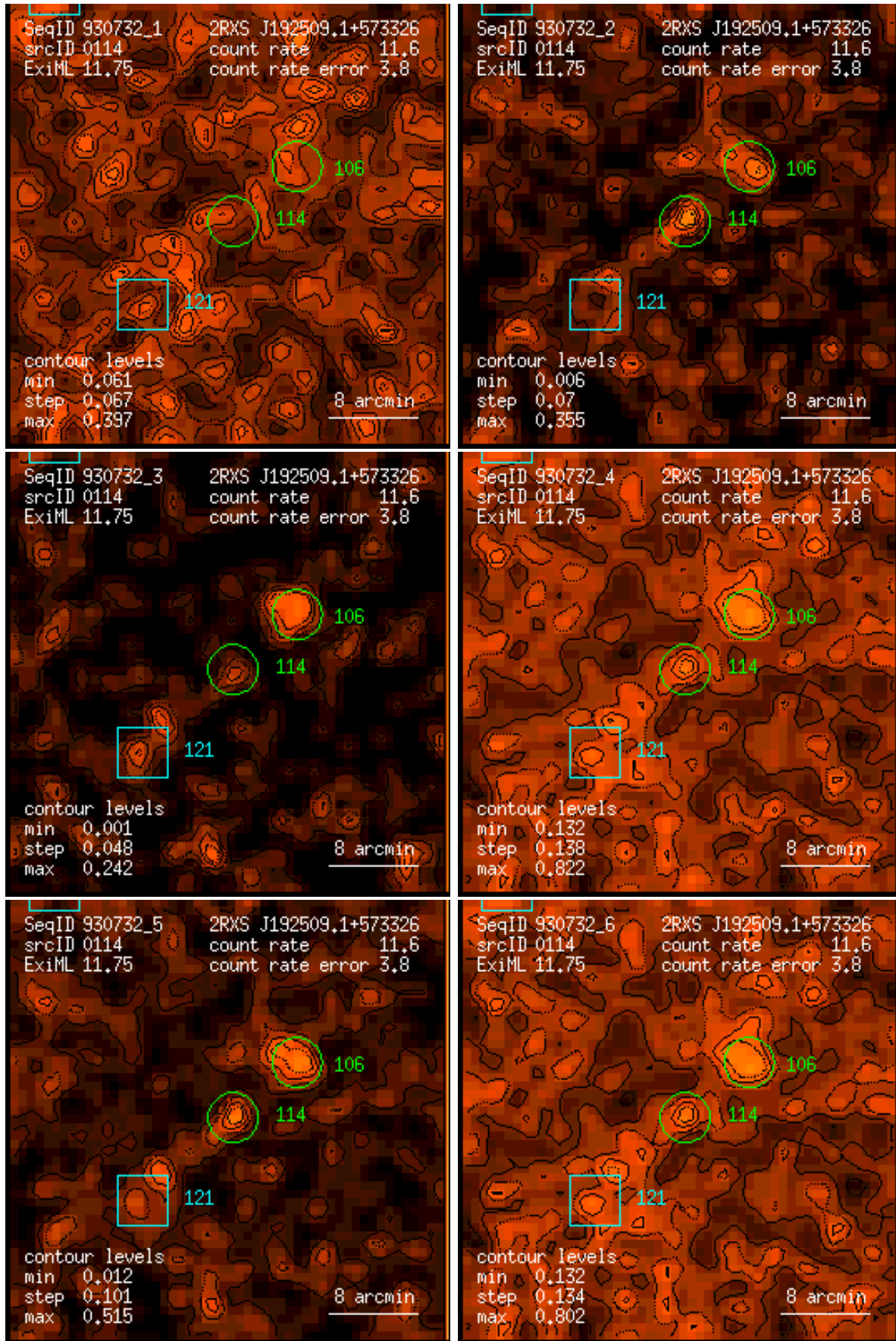
Figure 114: RASS 930732: detection 0114: band rate images, Gaussian filter: (1) PSPC channels 11 – 41, (2) 52 – 90, (3) 91 – 201, (4) 11 – 235, (5) 52 – 201, (6) 11 – 201. Broad band rates in counts/ks. Band rate contour levels in counts/ks/arcmin 2 .
