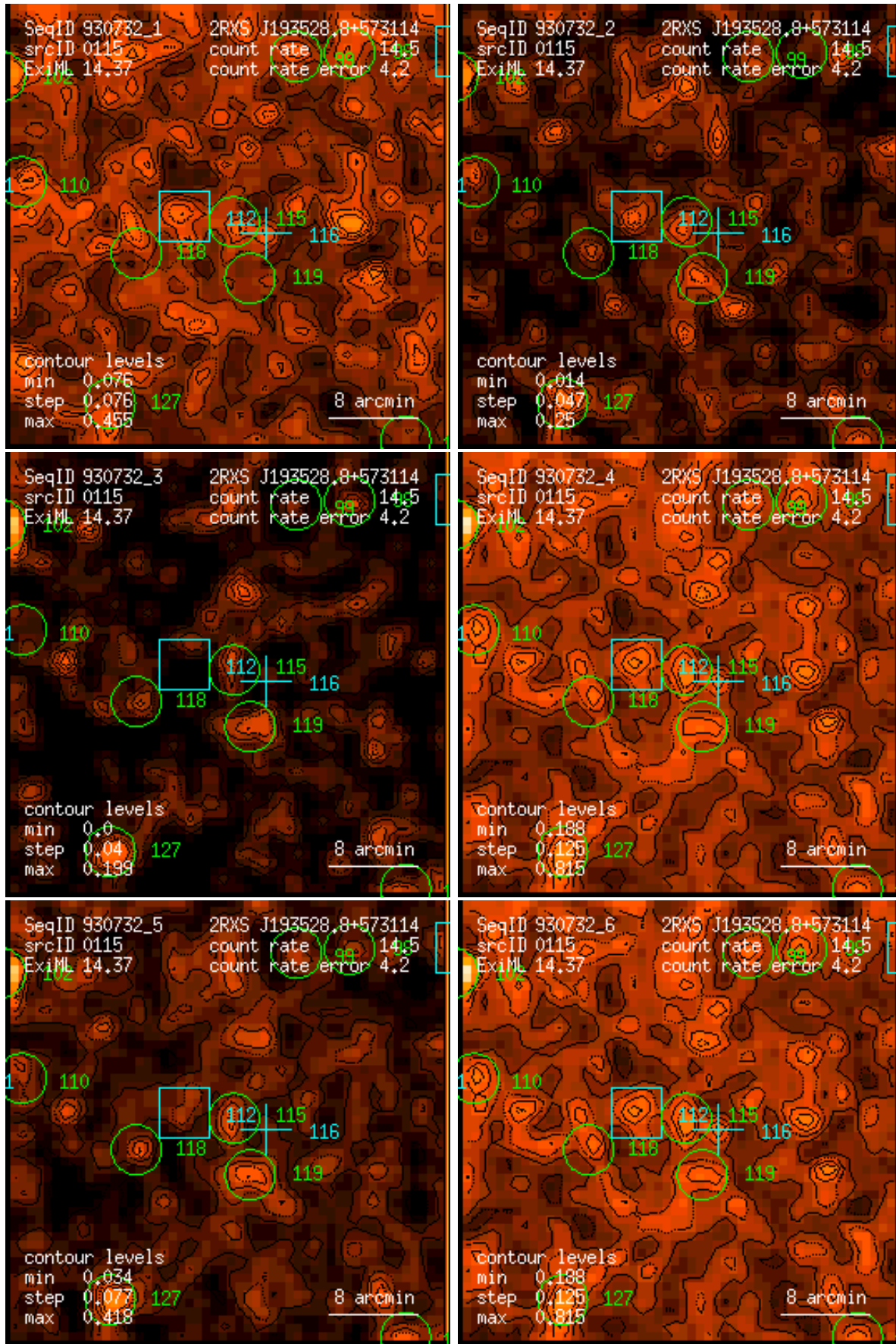
Figure 115: RASS 930732: detection 0115: band rate images, Gaussian filter: (1) PSPC channels 11 – 41, (2) 52 – 90, (3) 91 – 201, (4) 11 – 235, (5) 52 – 201, (6) 11 – 201. Broad band rates in counts/ks. Band rate contour levels in counts/ks/arcmin 2 .
