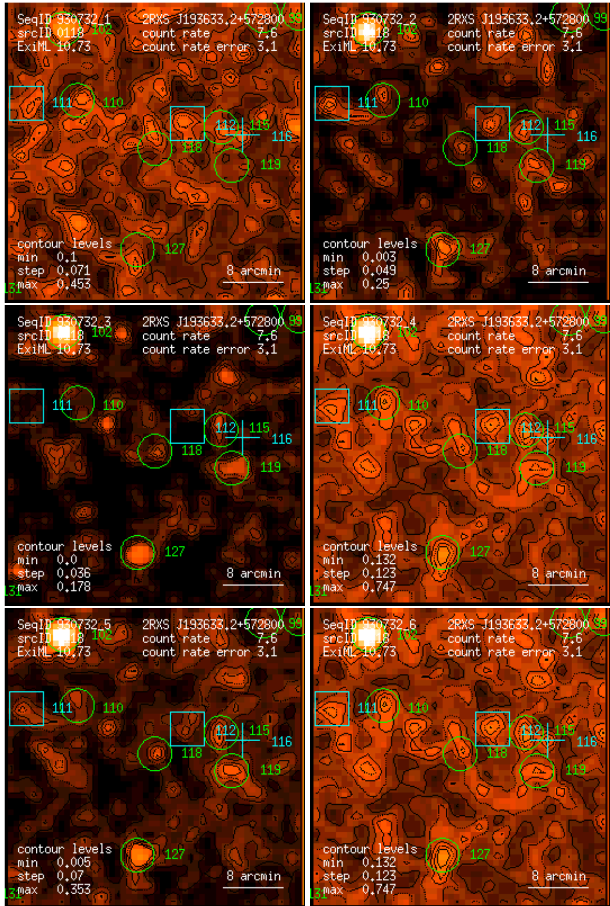
Figure 118: RASS 930732: detection 0118: band rate images, Gaussian filter: (1) PSPC channels 11 – 41, (2) 52 – 90, (3) 91 – 201, (4) 11 – 235, (5) 52 – 201, (6) 11 – 201. Broad band rates in counts/ks. Band rate contour levels in counts/ks/arcmin 2 .
