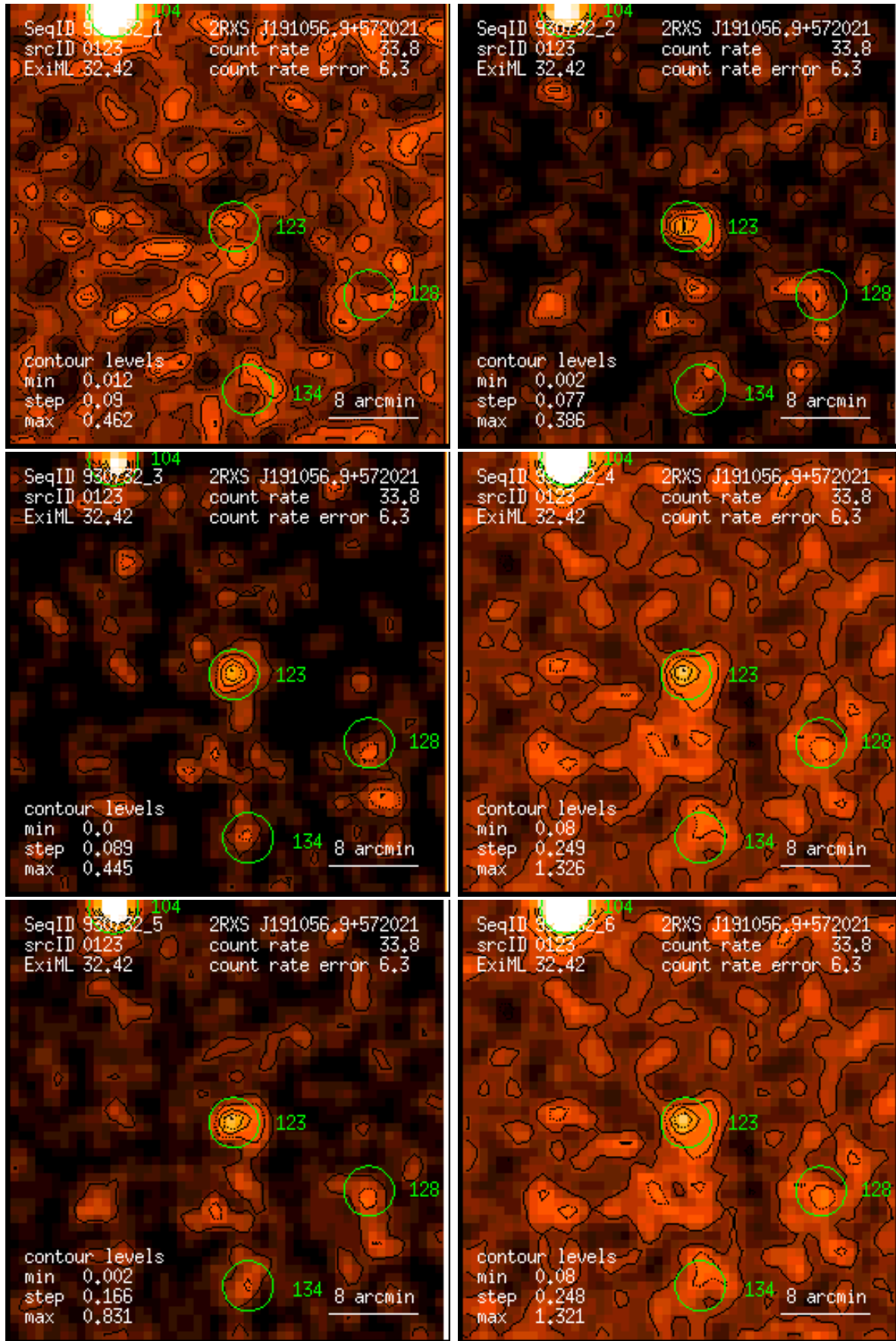
Figure 123: RASS 930732: detection 0123: band rate images, Gaussian filter: (1) PSPC channels 11 – 41, (2) 52 – 90, (3) 91 – 201, (4) 11 – 235, (5) 52 – 201, (6) 11 – 201. Broad band rates in counts/ks. Band rate contour levels in counts/ks/arcmin 2 .
