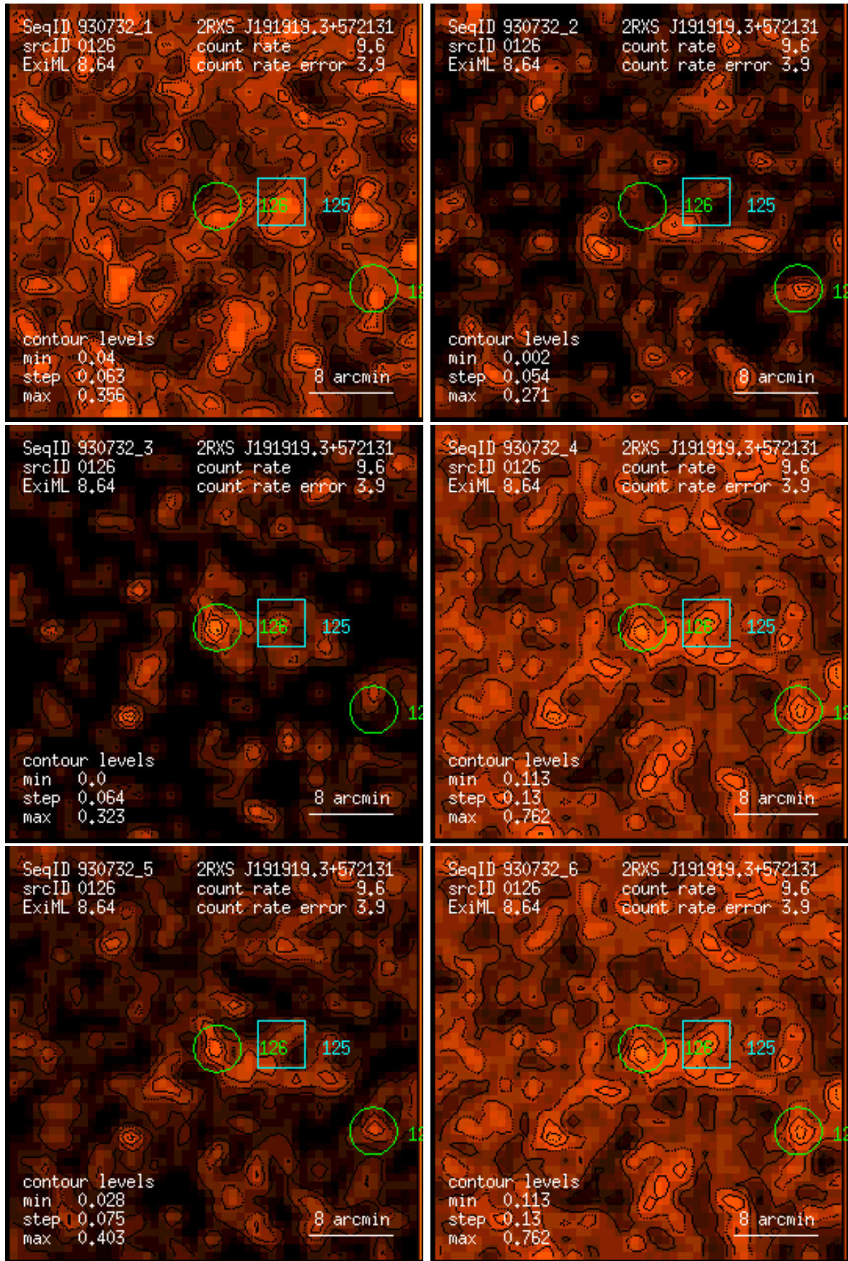
Figure 126: RASS 930732: detection 0126: band rate images, Gaussian filter: (1) PSPC channels 11 – 41, (2) 52 – 90, (3) 91 – 201, (4) 11 – 235, (5) 52 – 201, (6) 11 – 201. Broad band rates in counts/ks. Band rate contour levels in counts/ks/arcmin 2 .
