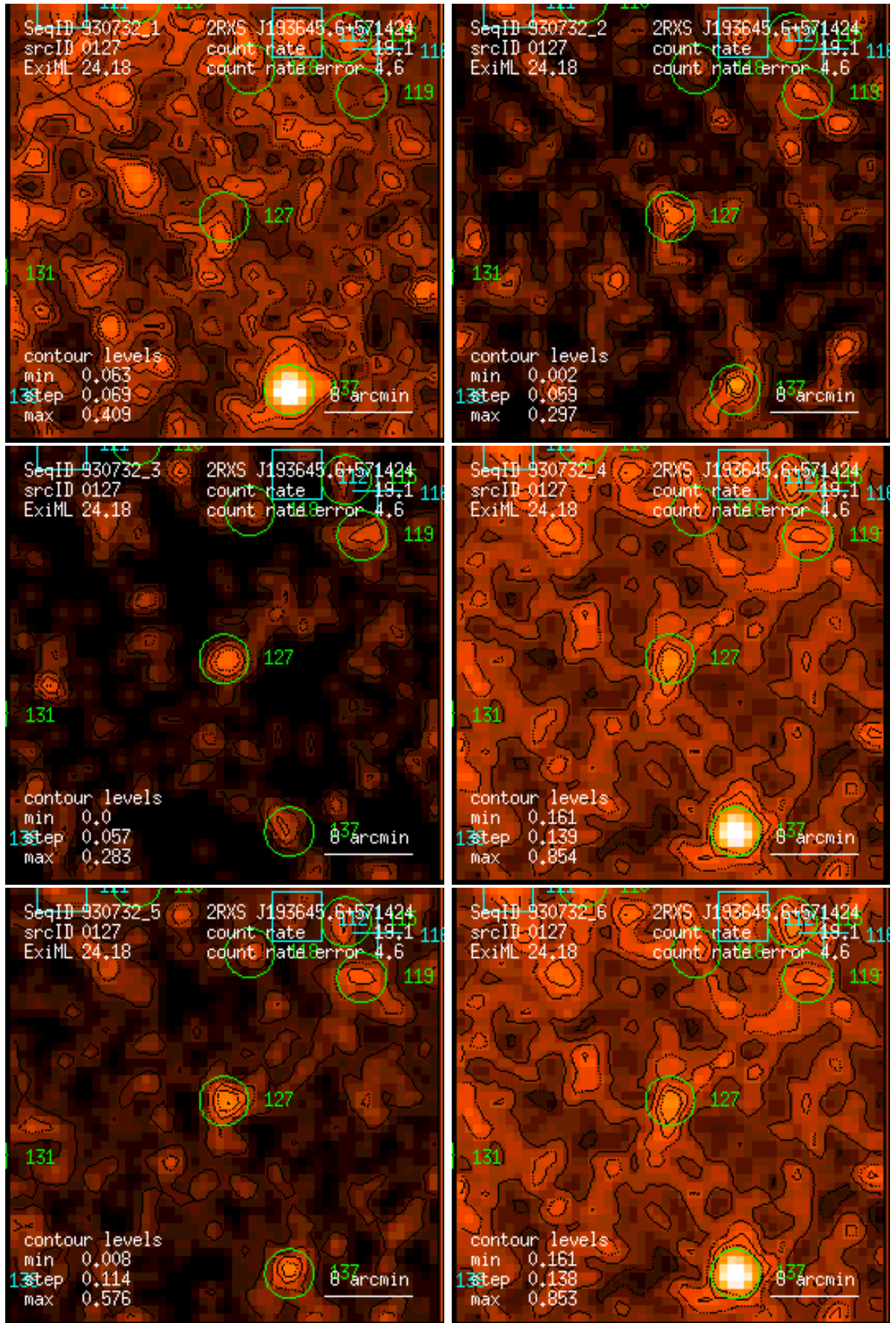
Figure 127: RASS 930732: detection 0127: band rate images, Gaussian filter: (1) PSPC channels 11 – 41, (2) 52 – 90, (3) 91 – 201, (4) 11 – 235, (5) 52 – 201, (6) 11 – 201. Broad band rates in counts/ks. Band rate contour levels in counts/ks/arcmin 2 .
