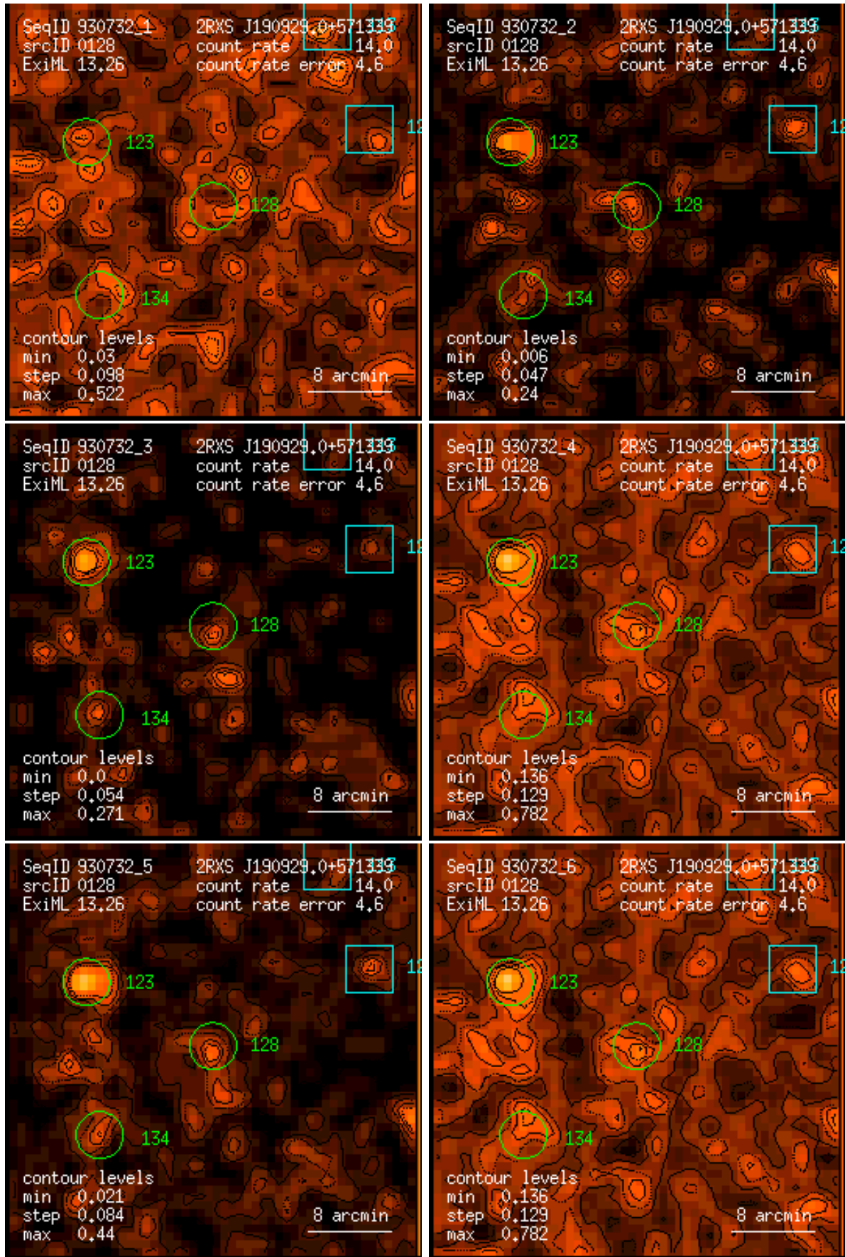
Figure 128: RASS 930732: detection 0128: band rate images, Gaussian filter: (1) PSPC channels 11 – 41, (2) 52 – 90, (3) 91 – 201, (4) 11 – 235, (5) 52 – 201, (6) 11 – 201. Broad band rates in counts/ks. Band rate contour levels in counts/ks/arcmin 2 .
