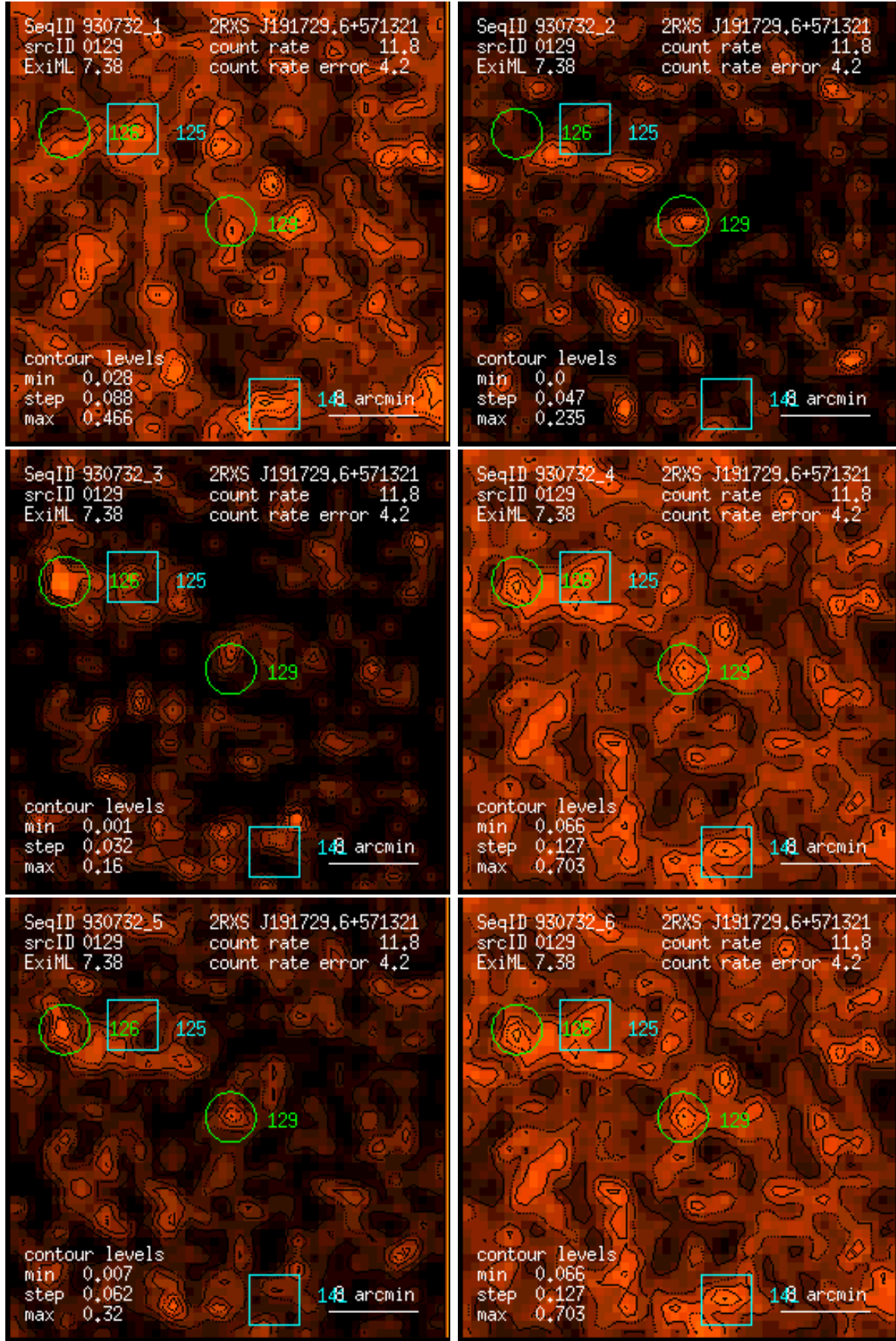
Figure 129: RASS 930732: detection 0129: band rate images, Gaussian filter: (1) PSPC channels 11 – 41, (2) 52 – 90, (3) 91 – 201, (4) 11 – 235, (5) 52 – 201, (6) 11 – 201. Broad band rates in counts/ks. Band rate contour levels in counts/ks/arcmin 2 .
