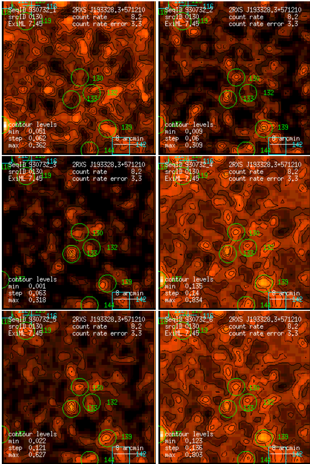
Figure 130: RASS 930732: detection 0130: band rate images, Gaussian filter: (1) PSPC channels 11 – 41, (2) 52 – 90, (3) 91 – 201, (4) 11 – 235, (5) 52 – 201, (6) 11 – 201. Broad band rates in counts/ks. Band rate contour levels in counts/ks/arcmin 2 .
