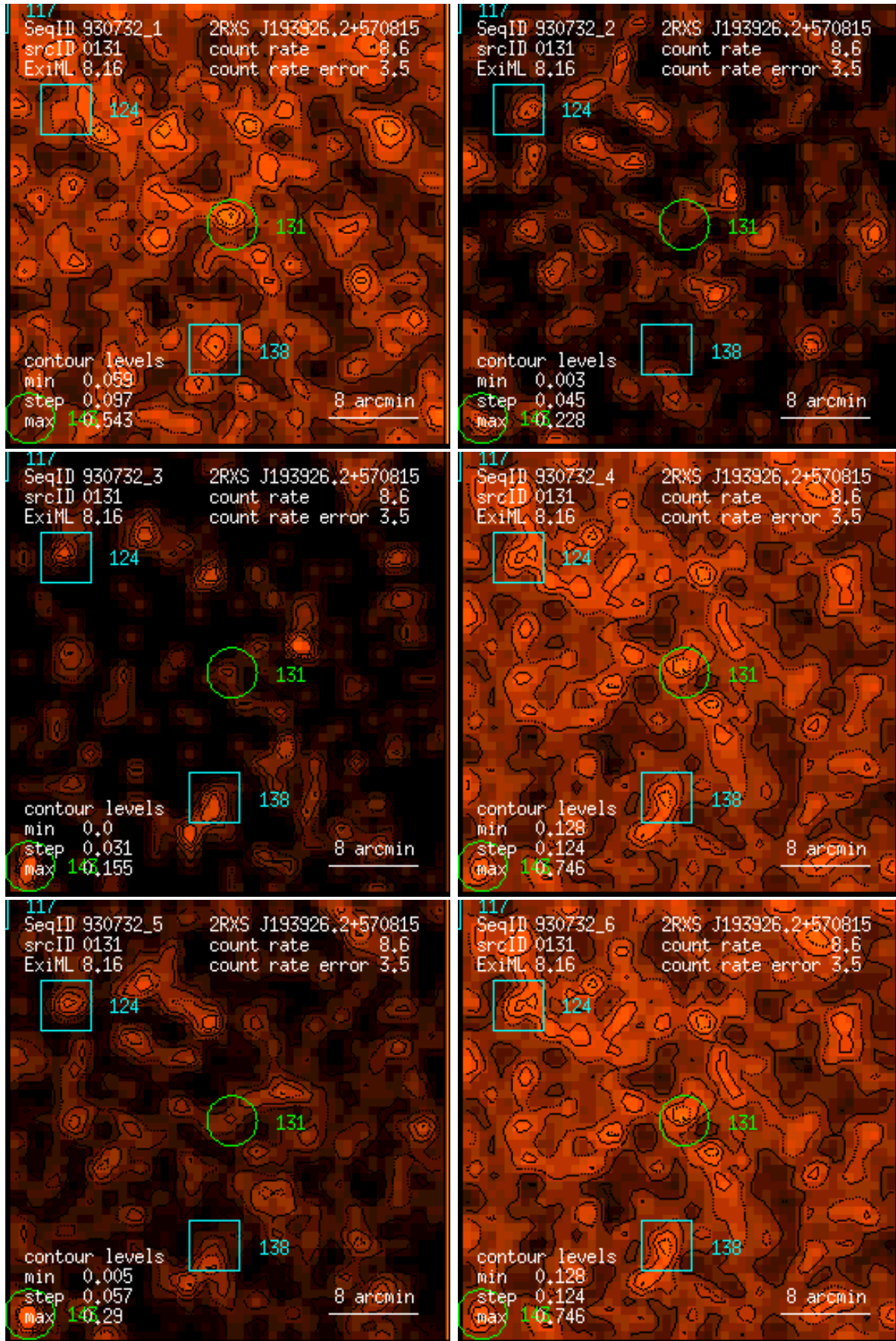
Figure 131: RASS 930732: detection 0131: band rate images, Gaussian filter: (1) PSPC channels 11 – 41, (2) 52 – 90, (3) 91 – 201, (4) 11 – 235, (5) 52 – 201, (6) 11 – 201. Broad band rates in counts/ks. Band rate contour levels in counts/ks/arcmin 2 .
