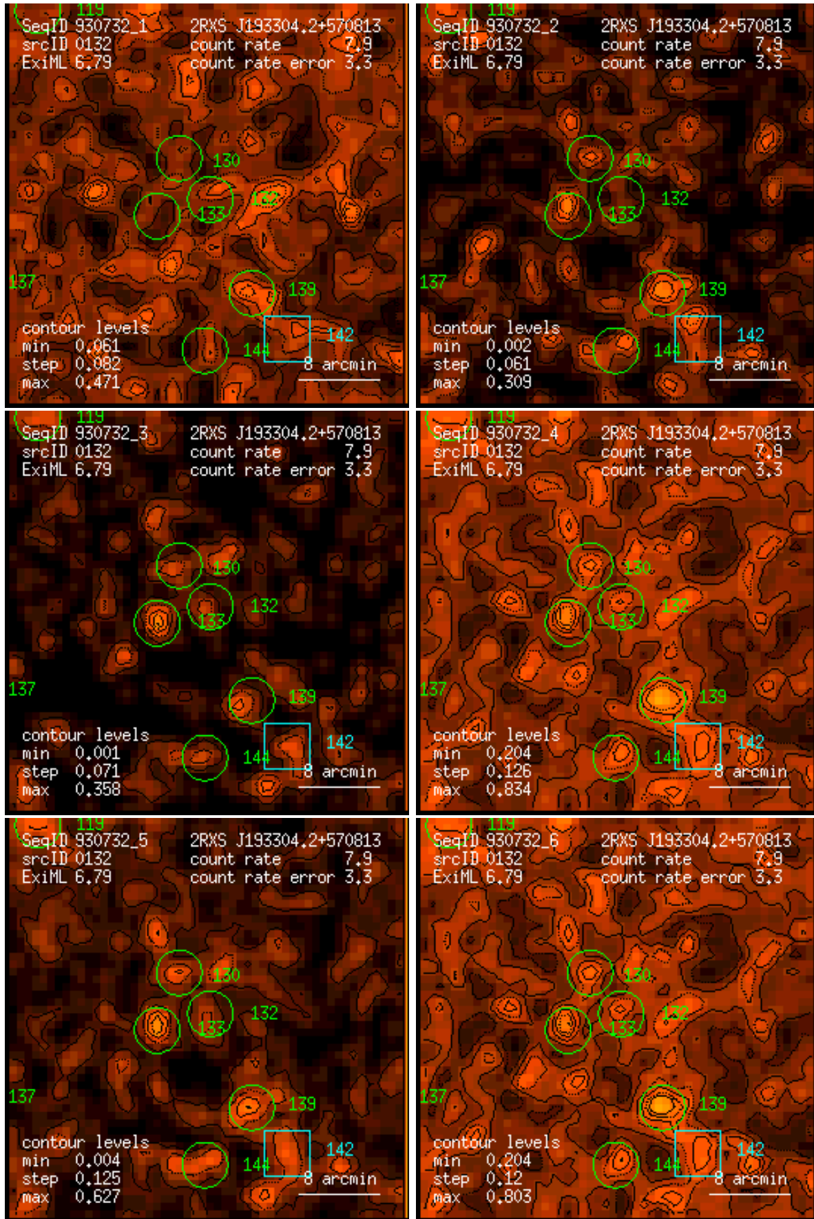
Figure 132: RASS 930732: detection 0132: band rate images, Gaussian filter: (1) PSPC channels 11 – 41, (2) 52 – 90, (3) 91 – 201, (4) 11 – 235, (5) 52 – 201, (6) 11 – 201. Broad band rates in counts/ks. Band rate contour levels in counts/ks/arcmin 2 .
