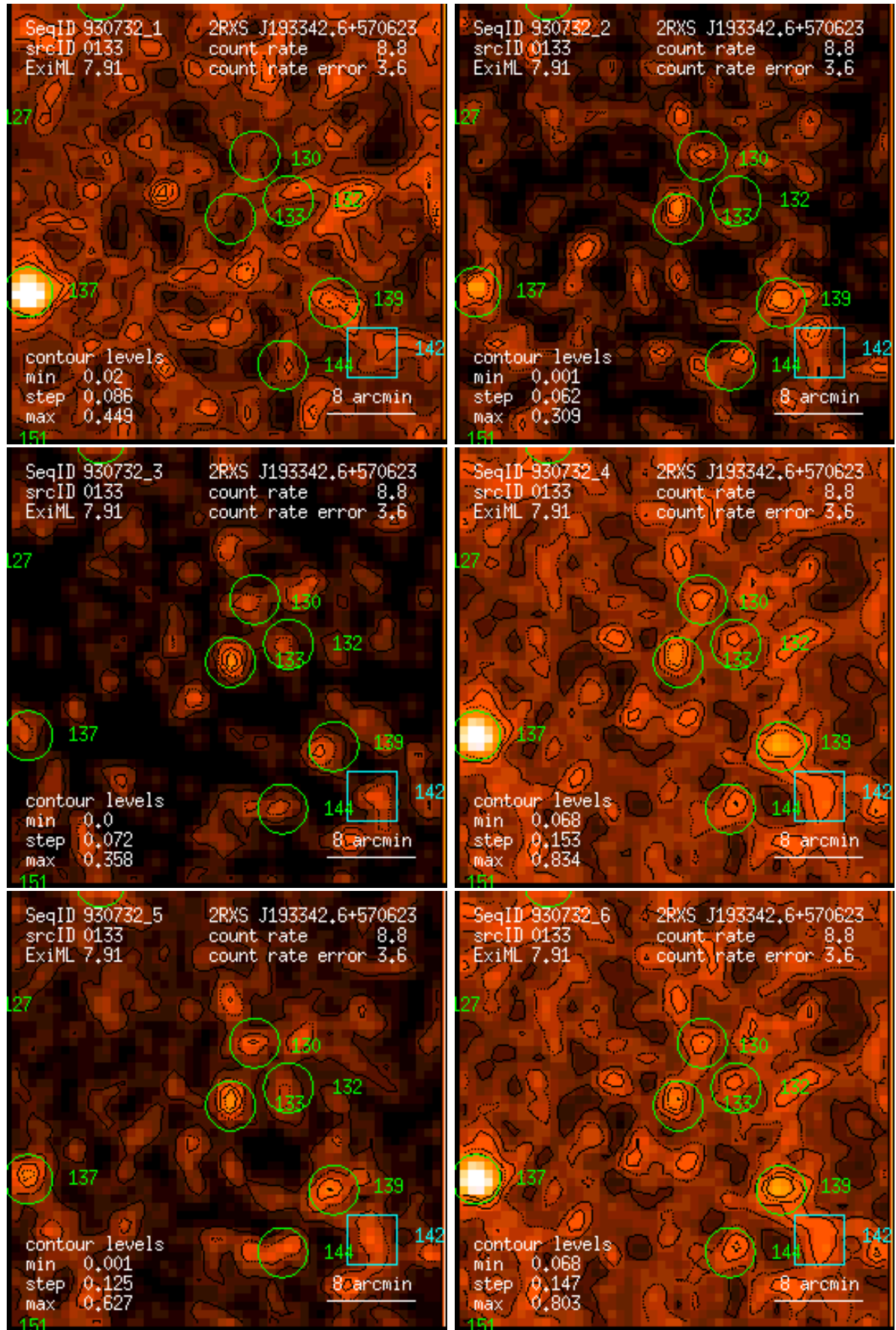
Figure 133: RASS 930732: detection 0133: band rate images, Gaussian filter: (1) PSPC channels 11 – 41, (2) 52 – 90, (3) 91 – 201, (4) 11 – 235, (5) 52 – 201, (6) 11 – 201. Broad band rates in counts/ks. Band rate contour levels in counts/ks/arcmin 2 .
