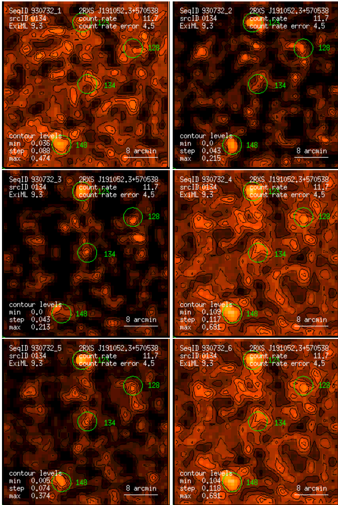
Figure 134: RASS 930732: detection 0134: band rate images, Gaussian filter: (1) PSPC channels 11 – 41, (2) 52 – 90, (3) 91 – 201, (4) 11 – 235, (5) 52 – 201, (6) 11 – 201. Broad band rates in counts/ks. Band rate contour levels in counts/ks/arcmin 2 .
