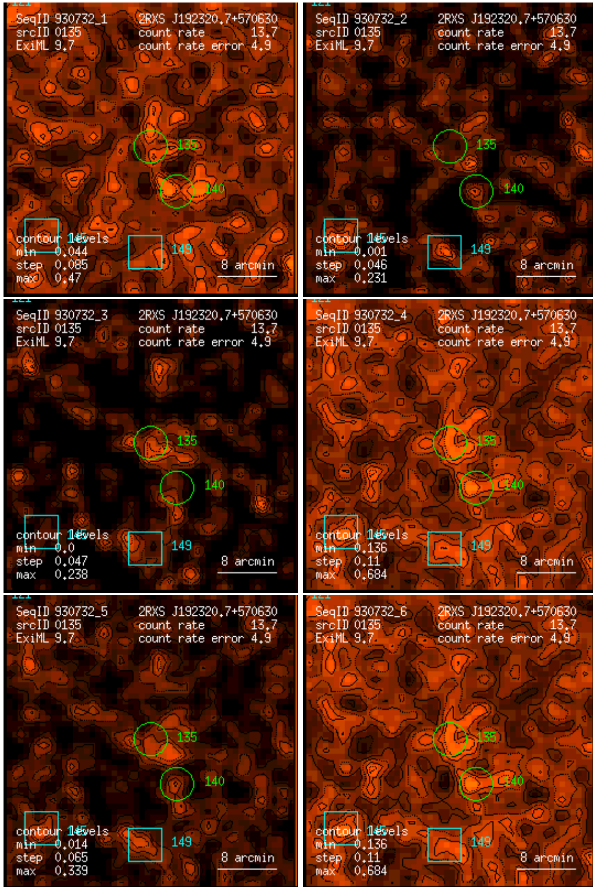
Figure 135: RASS 930732: detection 0135: band rate images, Gaussian filter: (1) PSPC channels 11 – 41, (2) 52 – 90, (3) 91 – 201, (4) 11 – 235, (5) 52 – 201, (6) 11 – 201. Broad band rates in counts/ks. Band rate contour levels in counts/ks/arcmin 2 .
