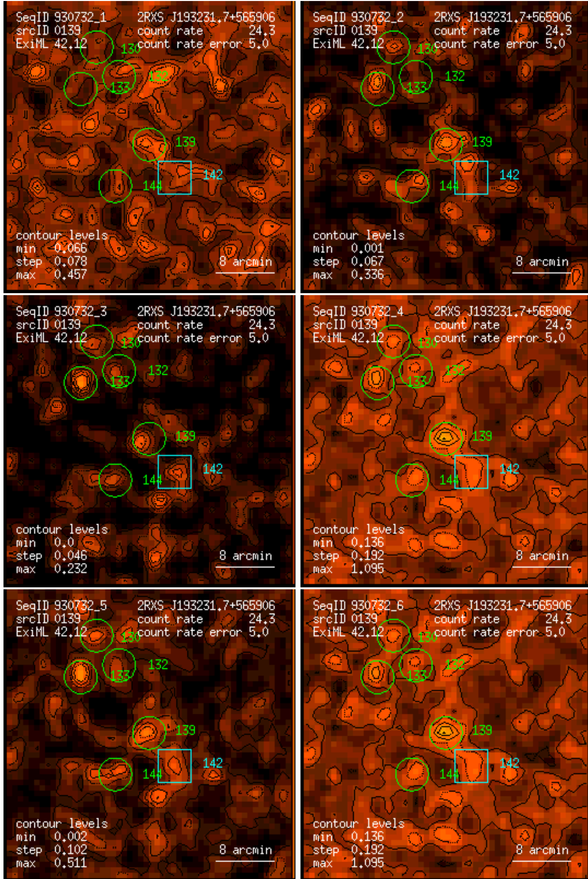
Figure 139: RASS 930732: detection 0139: band rate images, Gaussian filter: (1) PSPC channels 11 – 41, (2) 52 – 90, (3) 91 – 201, (4) 11 – 235, (5) 52 – 201, (6) 11 – 201. Broad band rates in counts/ks. Band rate contour levels in counts/ks/arcmin 2 .
