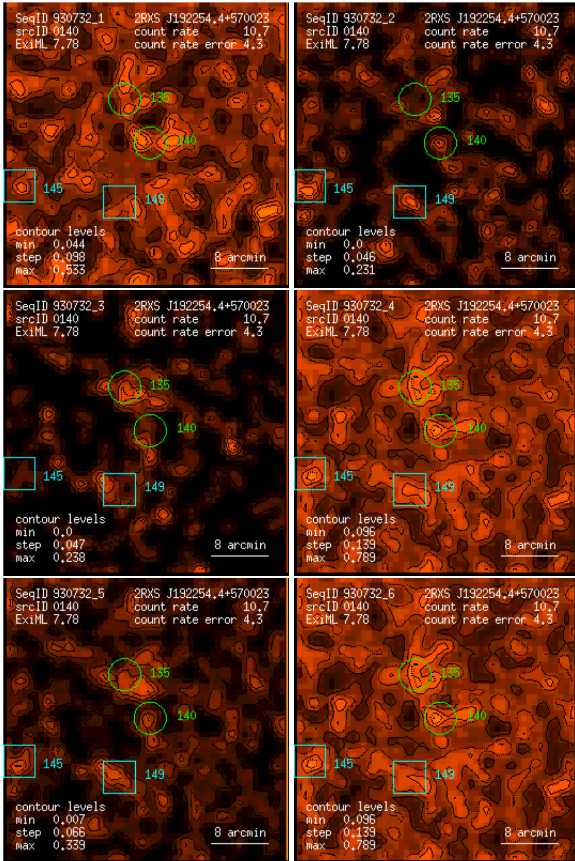
Figure 140: RASS 930732: detection 0140: band rate images, Gaussian filter: (1) PSPC channels 11 – 41, (2) 52 – 90, (3) 91 – 201, (4) 11 – 235, (5) 52 – 201, (6) 11 – 201. Broad band rates in counts/ks. Band rate contour levels in counts/ks/arcmin 2 .
