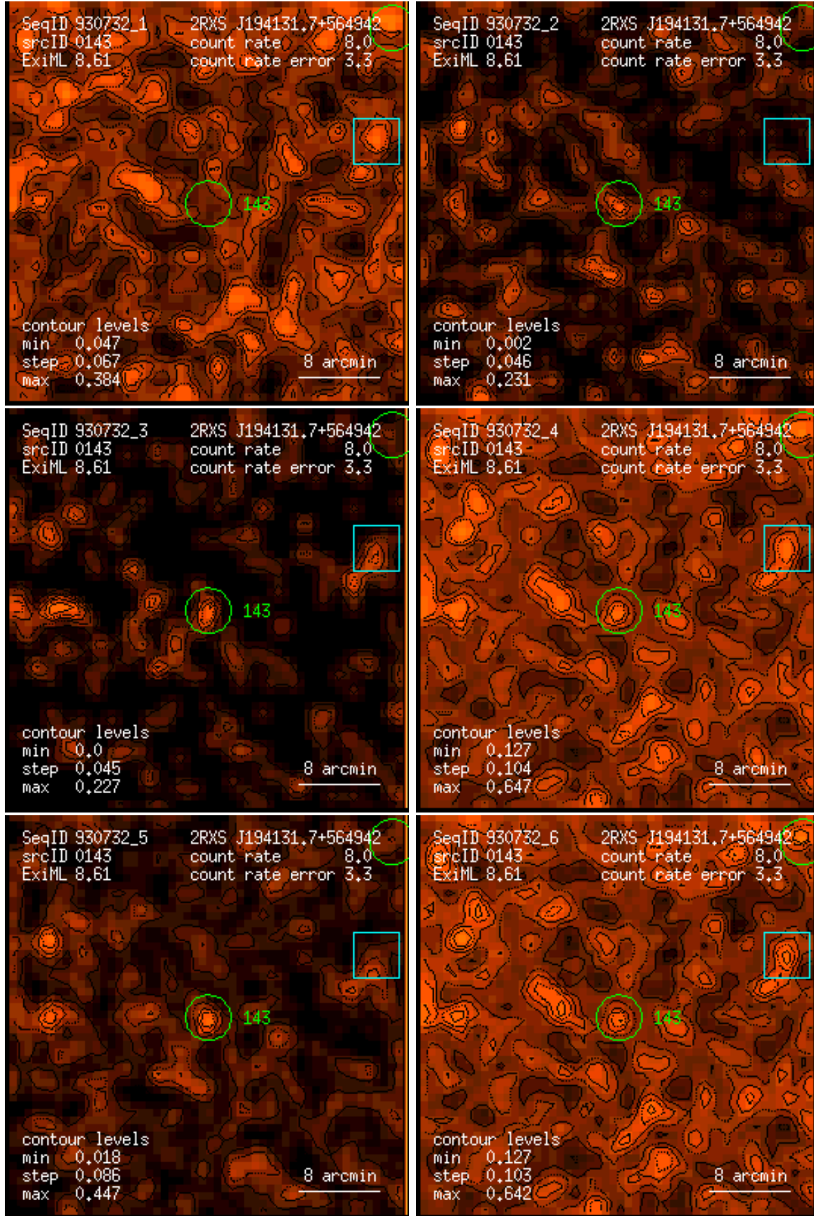
Figure 143: RASS 930732: detection 0143: band rate images, Gaussian filter: (1) PSPC channels 11 – 41, (2) 52 – 90, (3) 91 – 201, (4) 11 – 235, (5) 52 – 201, (6) 11 – 201. Broad band rates in counts/ks. Band rate contour levels in counts/ks/arcmin 2 .
