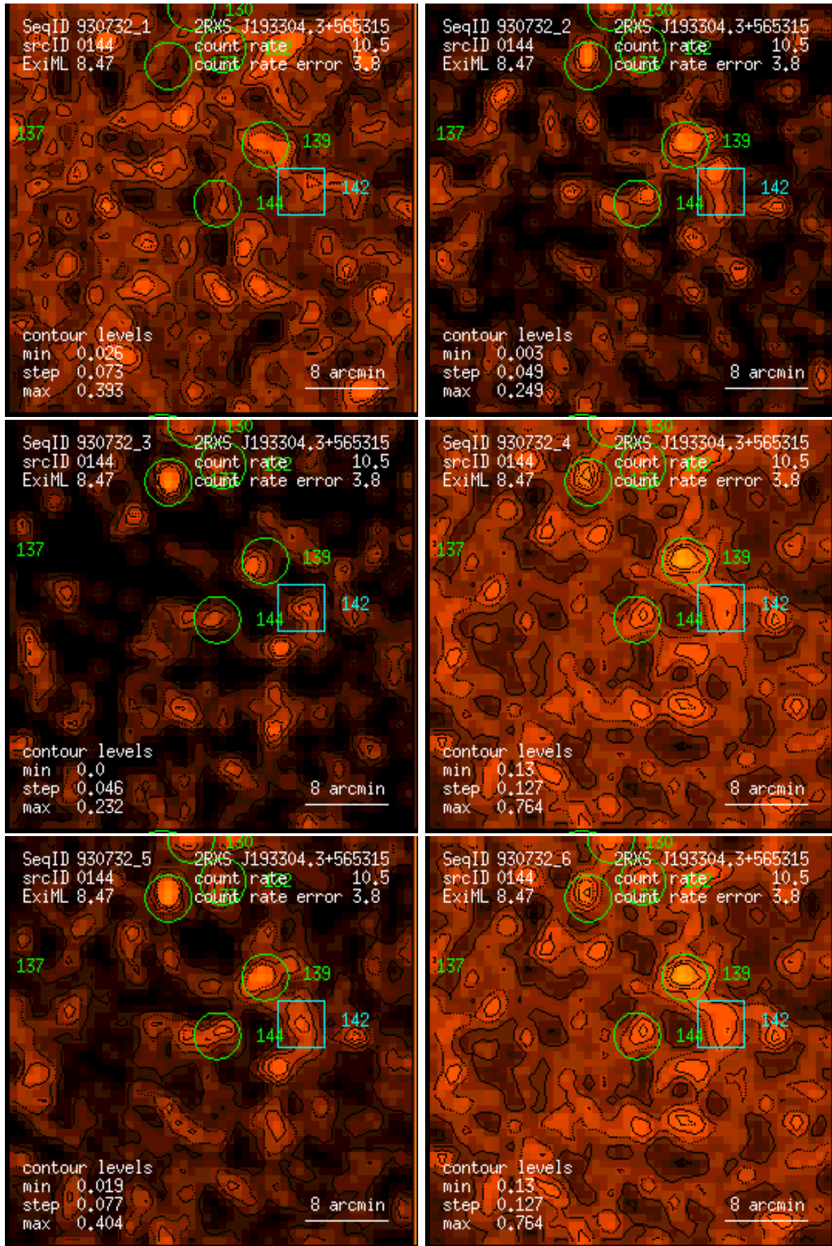
Figure 144: RASS 930732: detection 0144: band rate images, Gaussian filter: (1) PSPC channels 11 – 41, (2) 52 – 90, (3) 91 – 201, (4) 11 – 235, (5) 52 – 201, (6) 11 – 201. Broad band rates in counts/ks. Band rate contour levels in counts/ks/arcmin 2 .
