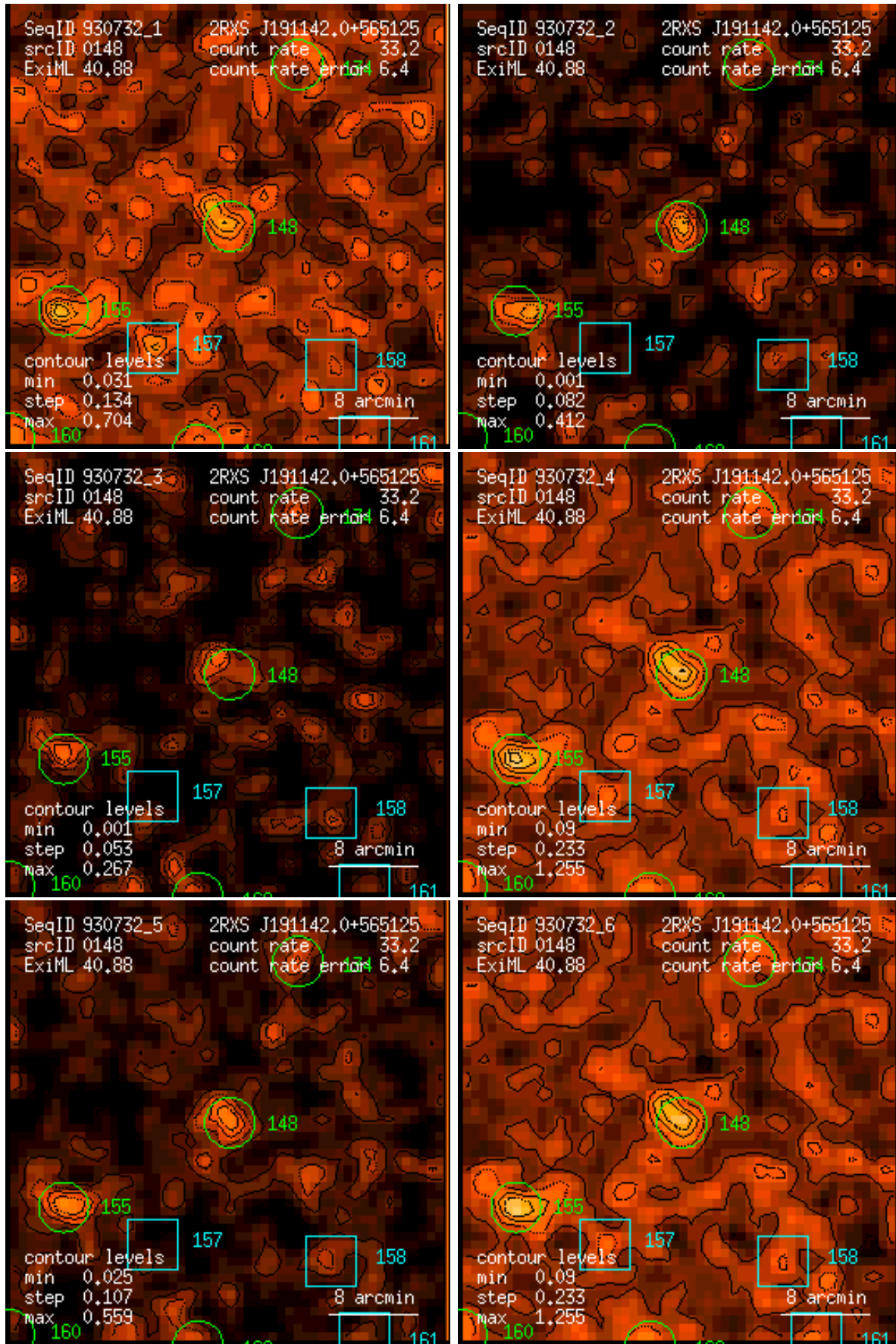
Figure 148: RASS 930732: detection 0148: band rate images, Gaussian filter: (1) PSPC channels 11 – 41, (2) 52 – 90, (3) 91 – 201, (4) 11 – 235, (5) 52 – 201, (6) 11 – 201. Broad band rates in counts/ks. Band rate contour levels in counts/ks/arcmin 2 .
