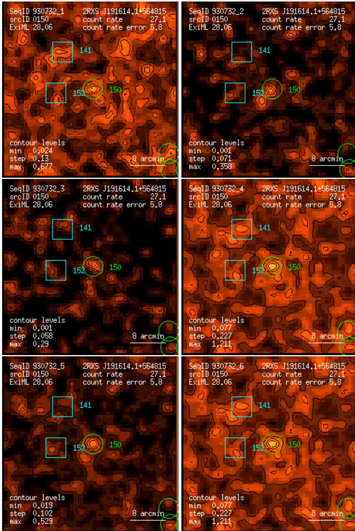
Figure 150: RASS 930732: detection 0150: band rate images, Gaussian filter: (1) PSPC channels 11 – 41, (2) 52 – 90, (3) 91 – 201, (4) 11 – 235, (5) 52 – 201, (6) 11 – 201. Broad band rates in counts/ks. Band rate contour levels in counts/ks/arcmin 2 .
