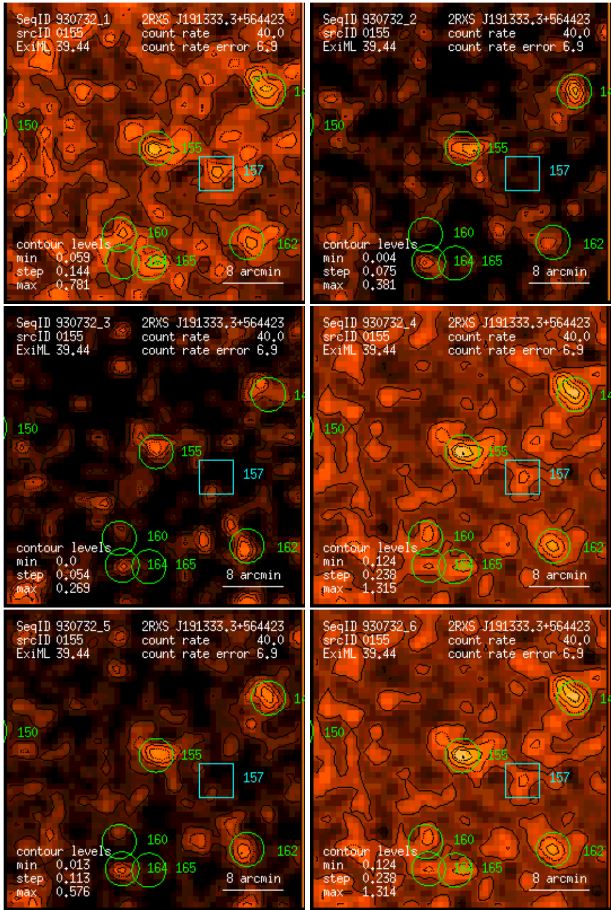
Figure 155: RASS 930732: detection 0155: band rate images, Gaussian filter: (1) PSPC channels 11 – 41, (2) 52 – 90, (3) 91 – 201, (4) 11 – 235, (5) 52 – 201, (6) 11 – 201. Broad band rates in counts/ks. Band rate contour levels in counts/ks/arcmin 2 .
