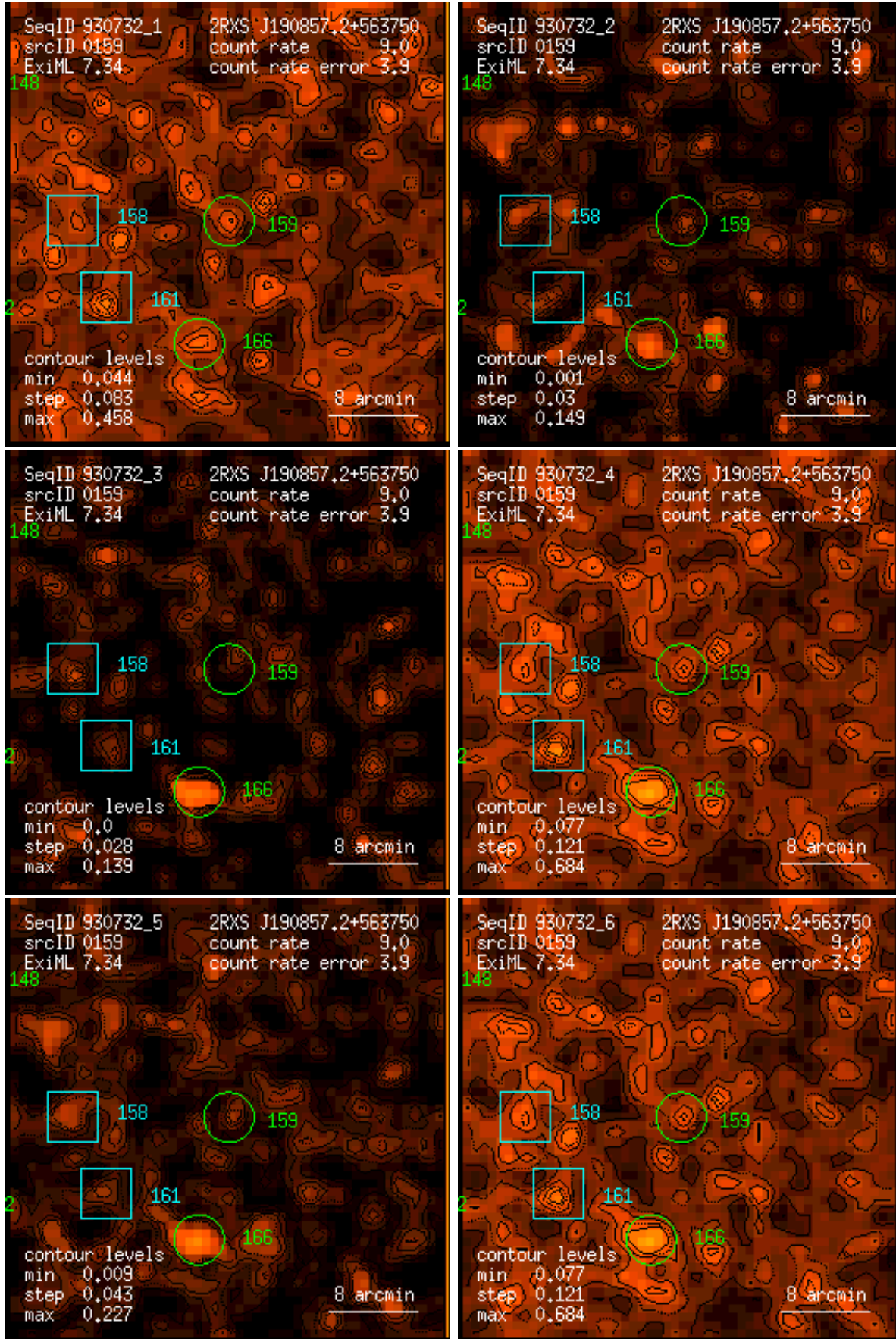
Figure 159: RASS 930732: detection 0159: band rate images, Gaussian filter: (1) PSPC channels 11 – 41, (2) 52 – 90, (3) 91 – 201, (4) 11 – 235, (5) 52 – 201, (6) 11 – 201. Broad band rates in counts/ks. Band rate contour levels in counts/ks/arcmin 2 .
