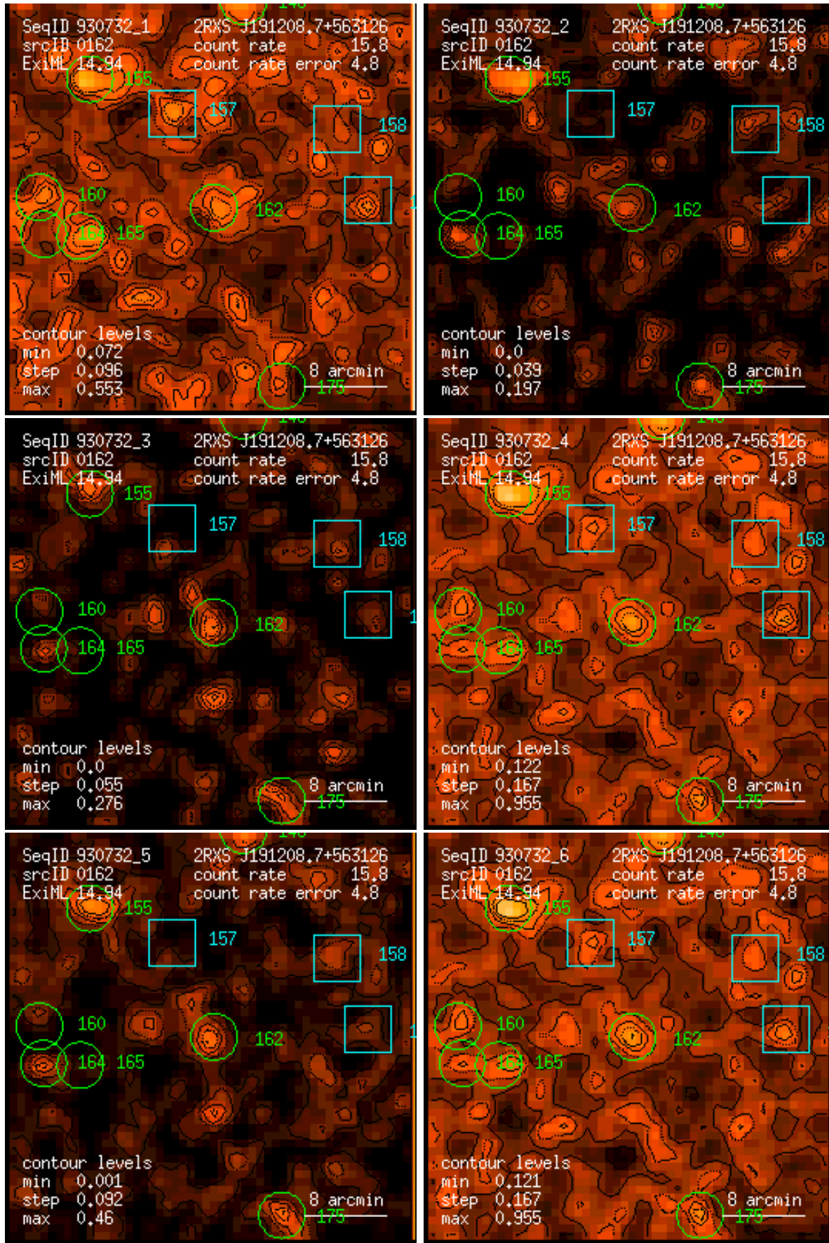
Figure 162: RASS 930732: detection 0162: band rate images, Gaussian filter: (1) PSPC channels 11 – 41, (2) 52 – 90, (3) 91 – 201, (4) 11 – 235, (5) 52 – 201, (6) 11 – 201. Broad band rates in counts/ks. Band rate contour levels in counts/ks/arcmin 2 .
