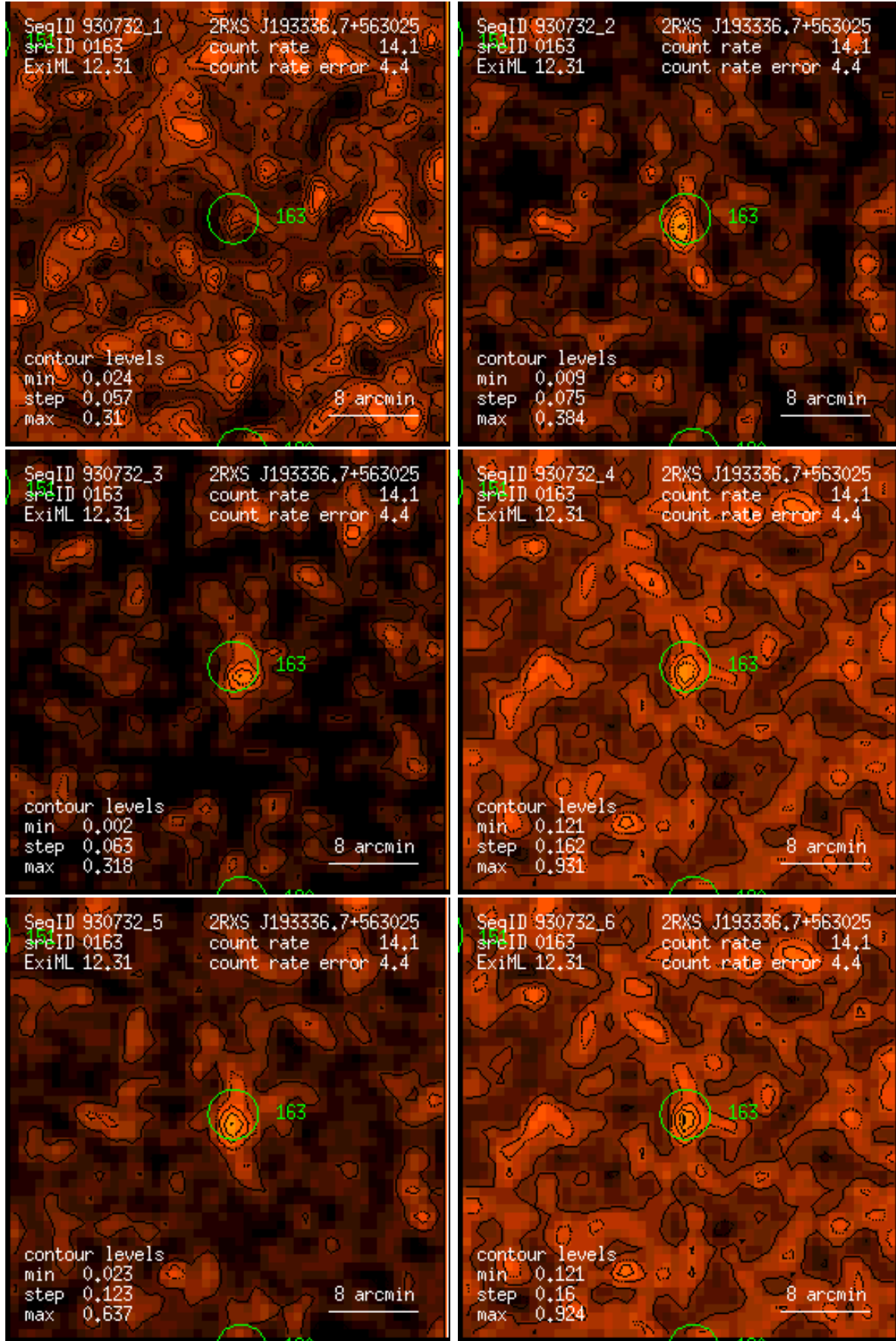
Figure 163: RASS 930732: detection 0163: band rate images, Gaussian filter: (1) PSPC channels 11 – 41, (2) 52 – 90, (3) 91 – 201, (4) 11 – 235, (5) 52 – 201, (6) 11 – 201. Broad band rates in counts/ks. Band rate contour levels in counts/ks/arcmin 2 .
