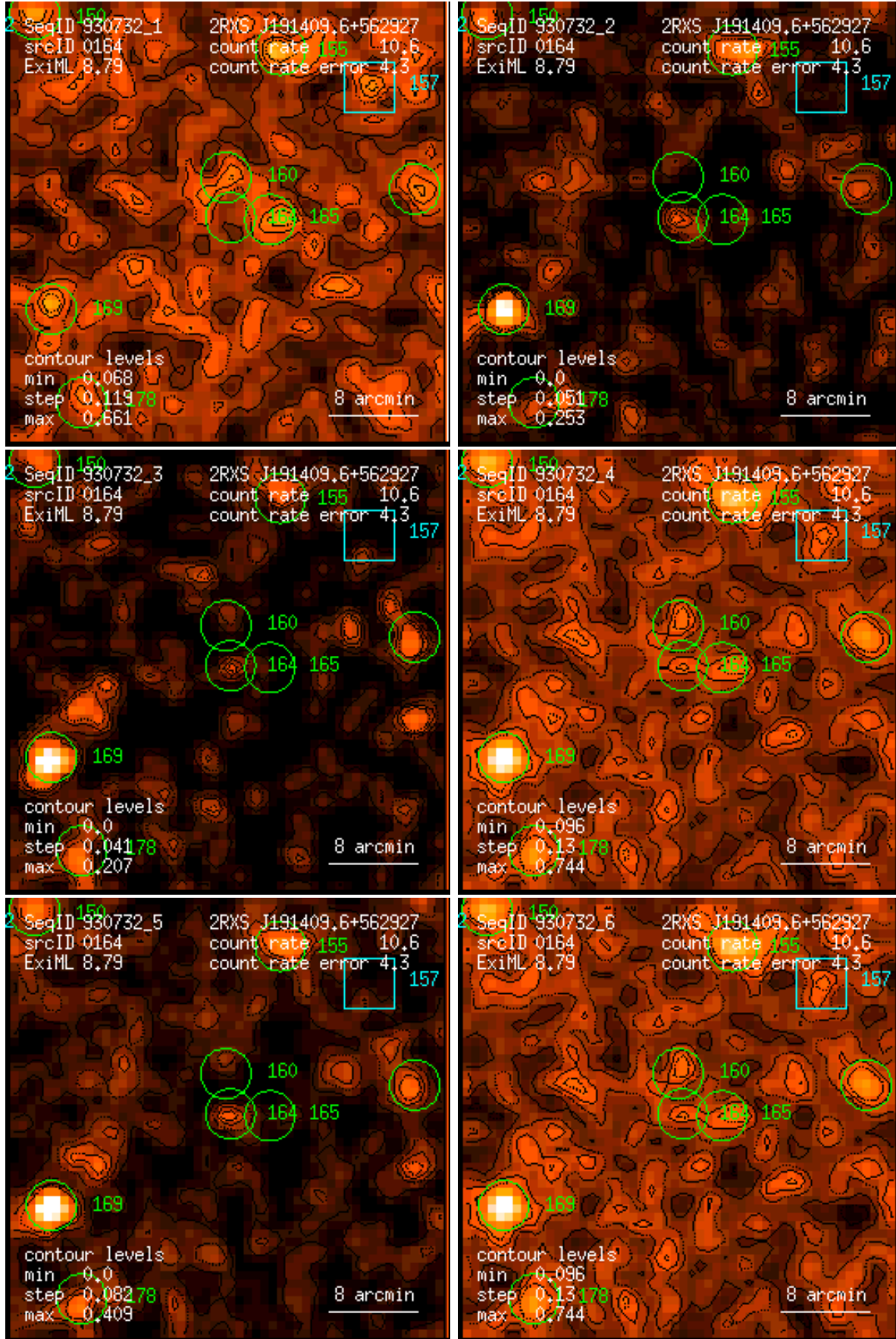
Figure 164: RASS 930732: detection 0164: band rate images, Gaussian filter: (1) PSPC channels 11 – 41, (2) 52 – 90, (3) 91 – 201, (4) 11 – 235, (5) 52 – 201, (6) 11 – 201. Broad band rates in counts/ks. Band rate contour levels in counts/ks/arcmin 2 .
