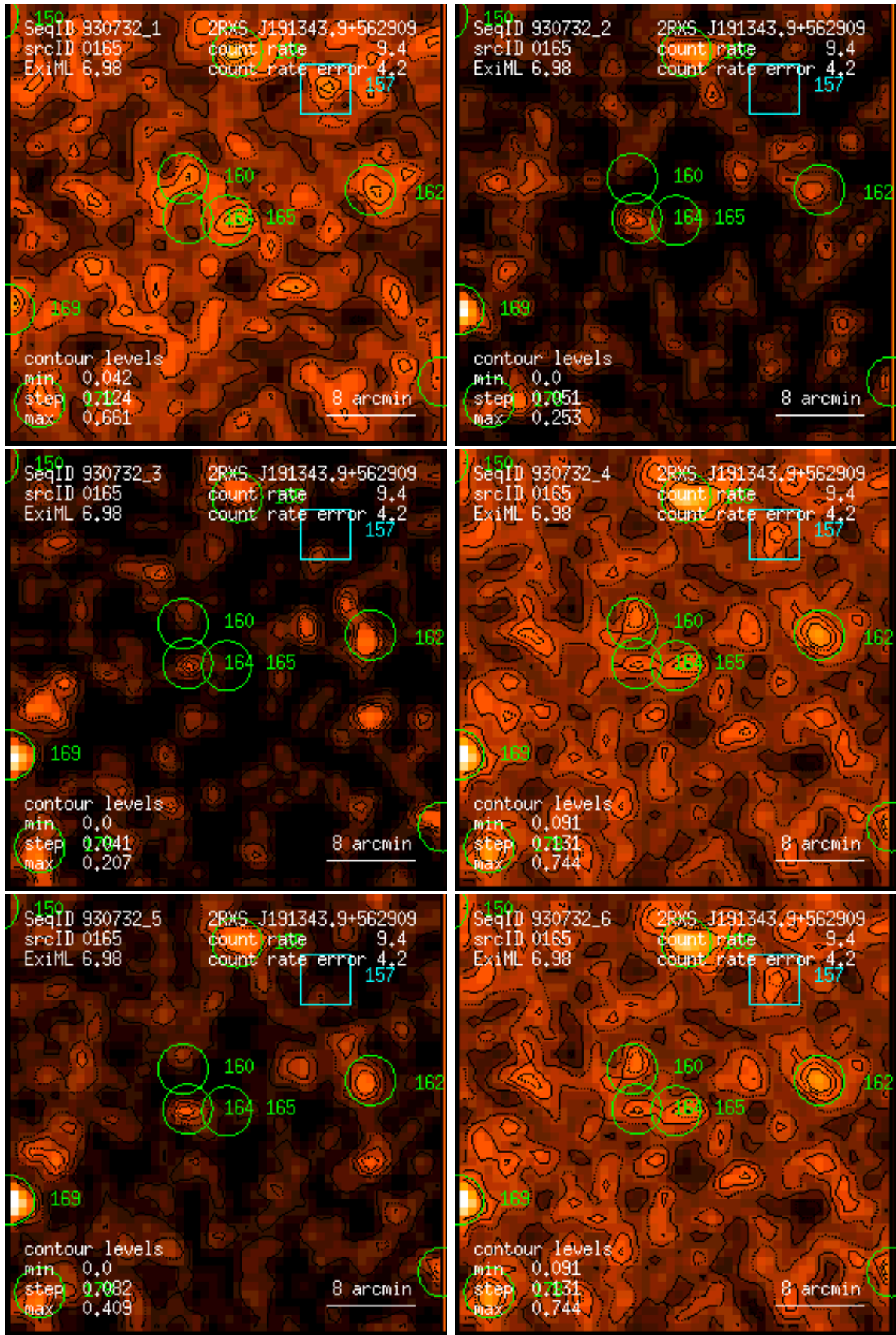
Figure 165: RASS 930732: detection 0165: band rate images, Gaussian filter: (1) PSPC channels 11 – 41, (2) 52 – 90, (3) 91 – 201, (4) 11 – 235, (5) 52 – 201, (6) 11 – 201. Broad band rates in counts/ks. Band rate contour levels in counts/ks/arcmin 2 .
