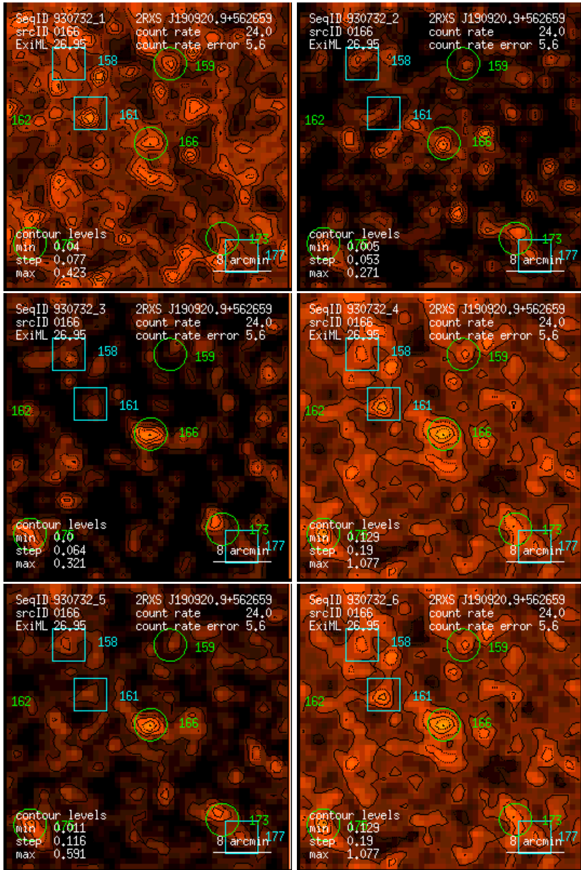
Figure 166: RASS 930732: detection 0166: band rate images, Gaussian filter: (1) PSPC channels 11 – 41, (2) 52 – 90, (3) 91 – 201, (4) 11 – 235, (5) 52 – 201, (6) 11 – 201. Broad band rates in counts/ks. Band rate contour levels in counts/ks/arcmin 2 .
