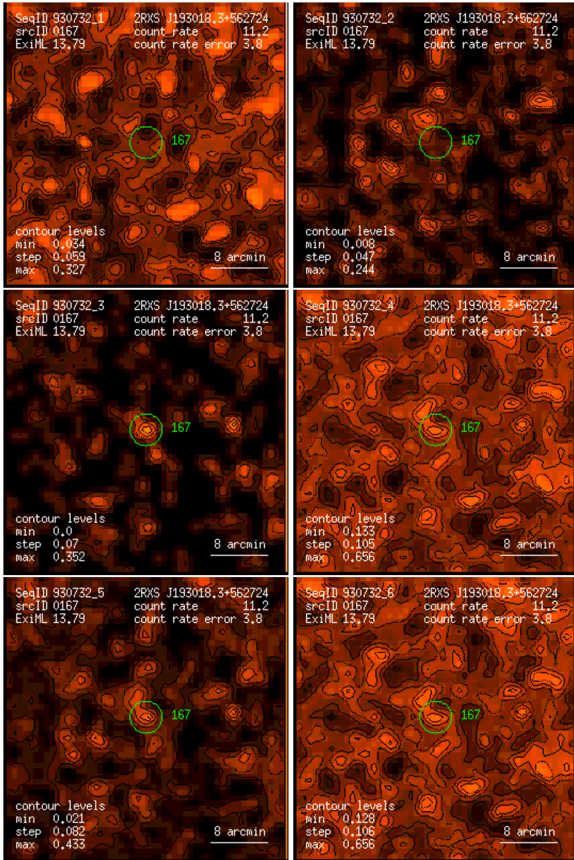
Figure 167: RASS 930732: detection 0167: band rate images, Gaussian filter: (1) PSPC channels 11 – 41, (2) 52 – 90, (3) 91 – 201, (4) 11 – 235, (5) 52 – 201, (6) 11 – 201. Broad band rates in counts/ks. Band rate contour levels in counts/ks/arcmin 2 .
