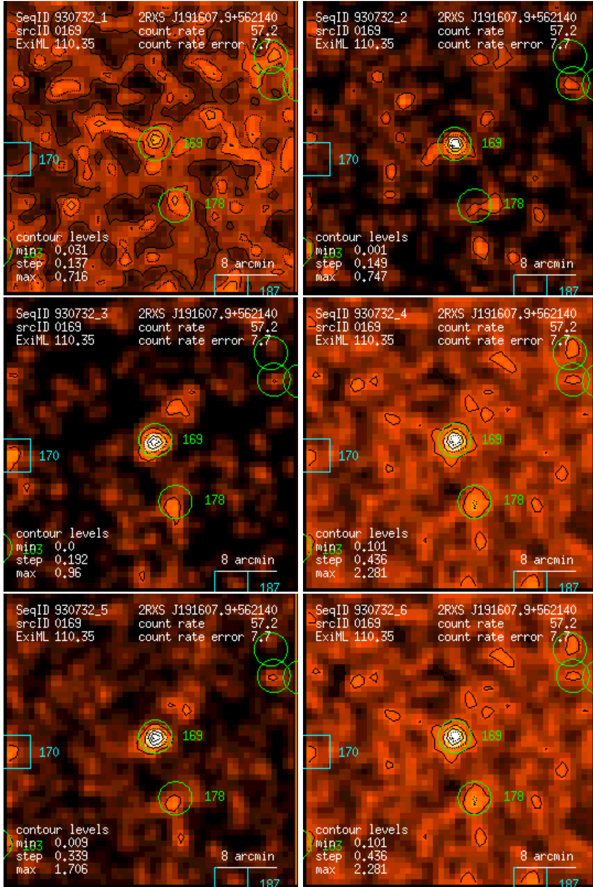
Figure 169: RASS 930732: detection 0169: band rate images, Gaussian filter: (1) PSPC channels 11 – 41, (2) 52 – 90, (3) 91 – 201, (4) 11 – 235, (5) 52 – 201, (6) 11 – 201. Broad band rates in counts/ks. Band rate contour levels in counts/ks/arcmin 2 .
