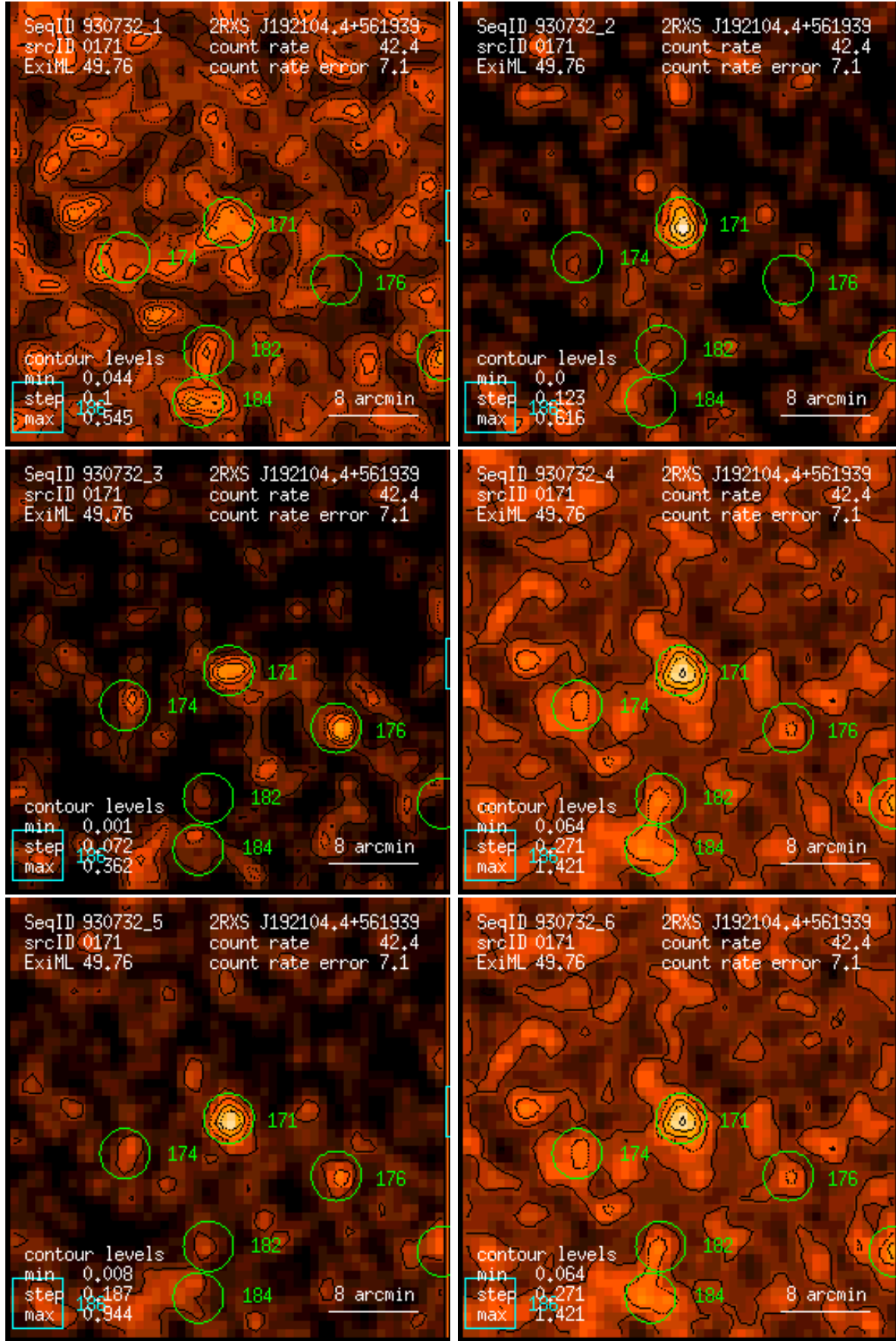
Figure 171: RASS 930732: detection 0171: band rate images, Gaussian filter: (1) PSPC channels 11 – 41, (2) 52 – 90, (3) 91 – 201, (4) 11 – 235, (5) 52 – 201, (6) 11 – 201. Broad band rates in counts/ks. Band rate contour levels in counts/ks/arcmin 2 .
