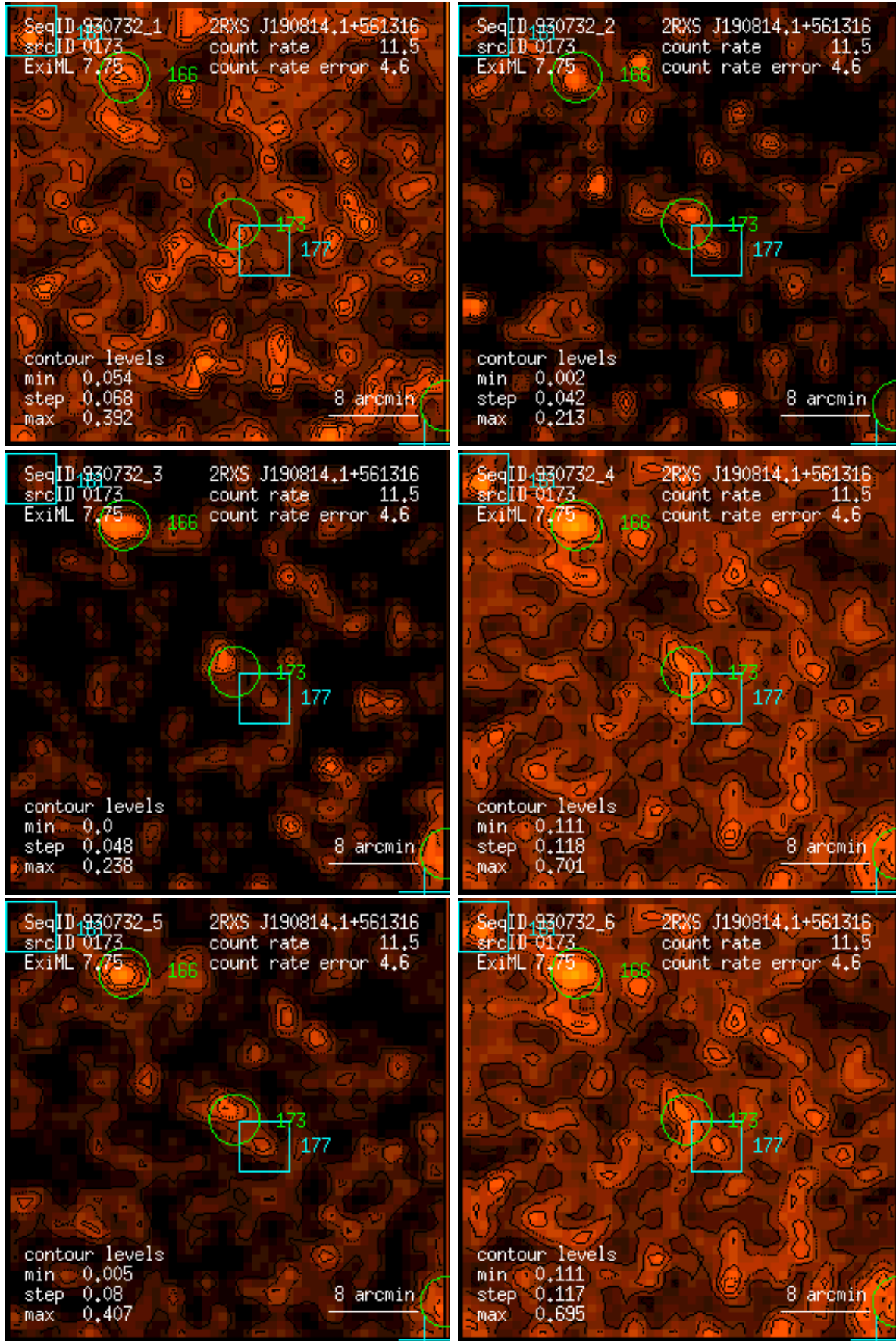
Figure 173: RASS 930732: detection 0173: band rate images, Gaussian filter: (1) PSPC channels 11 – 41, (2) 52 – 90, (3) 91 – 201, (4) 11 – 235, (5) 52 – 201, (6) 11 – 201. Broad band rates in counts/ks. Band rate contour levels in counts/ks/arcmin 2 .
