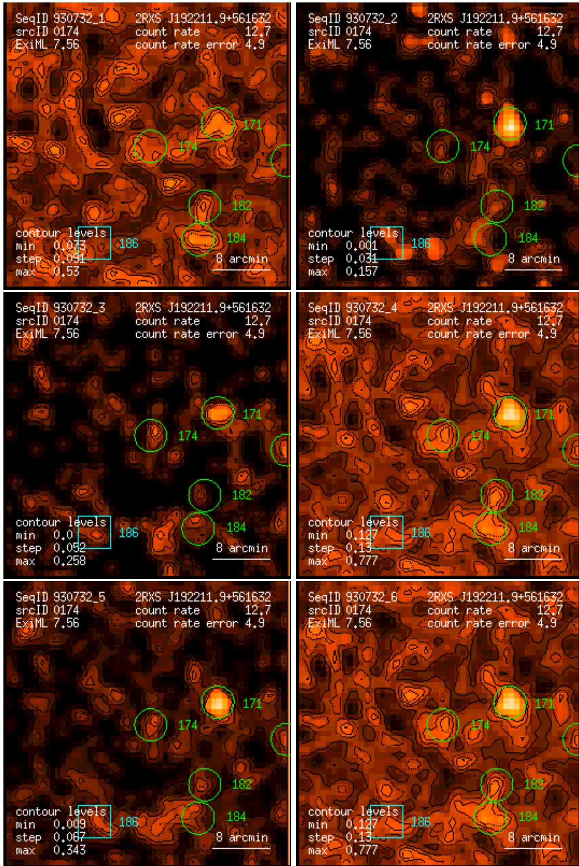
Figure 174: RASS 930732: detection 0174: band rate images, Gaussian filter: (1) PSPC channels 11 – 41, (2) 52 – 90, (3) 91 – 201, (4) 11 – 235, (5) 52 – 201, (6) 11 – 201. Broad band rates in counts/ks. Band rate contour levels in counts/ks/arcmin 2 .
