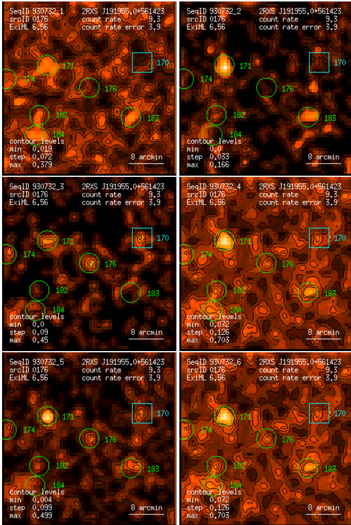
Figure 176: RASS 930732: detection 0176: band rate images, Gaussian filter: (1) PSPC channels 11 – 41, (2) 52 – 90, (3) 91 – 201, (4) 11 – 235, (5) 52 – 201, (6) 11 – 201. Broad band rates in counts/ks. Band rate contour levels in counts/ks/arcmin 2 .
