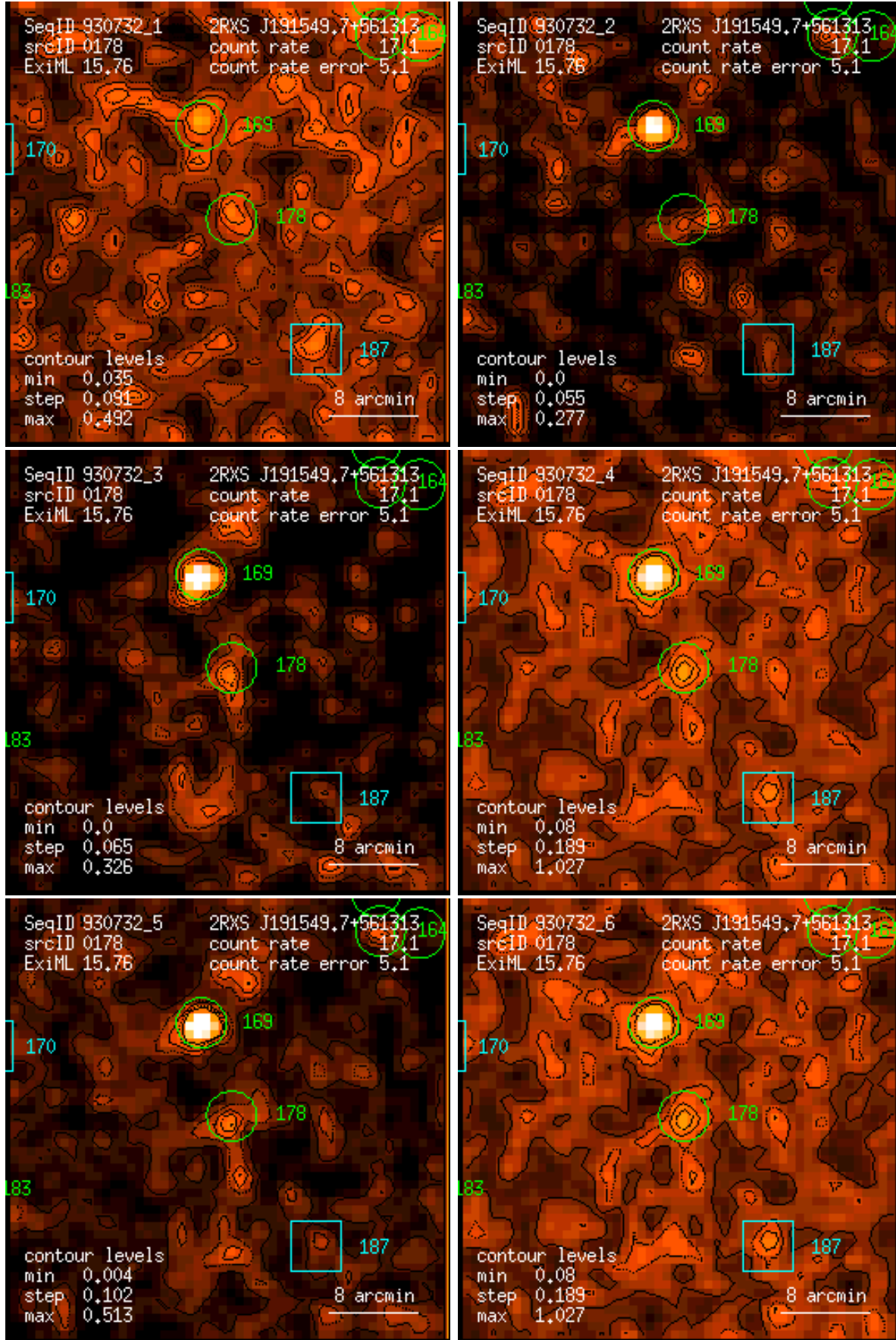
Figure 178: RASS 930732: detection 0178: band rate images, Gaussian filter: (1) PSPC channels 11 – 41, (2) 52 – 90, (3) 91 – 201, (4) 11 – 235, (5) 52 – 201, (6) 11 – 201. Broad band rates in counts/ks. Band rate contour levels in counts/ks/arcmin 2 .
