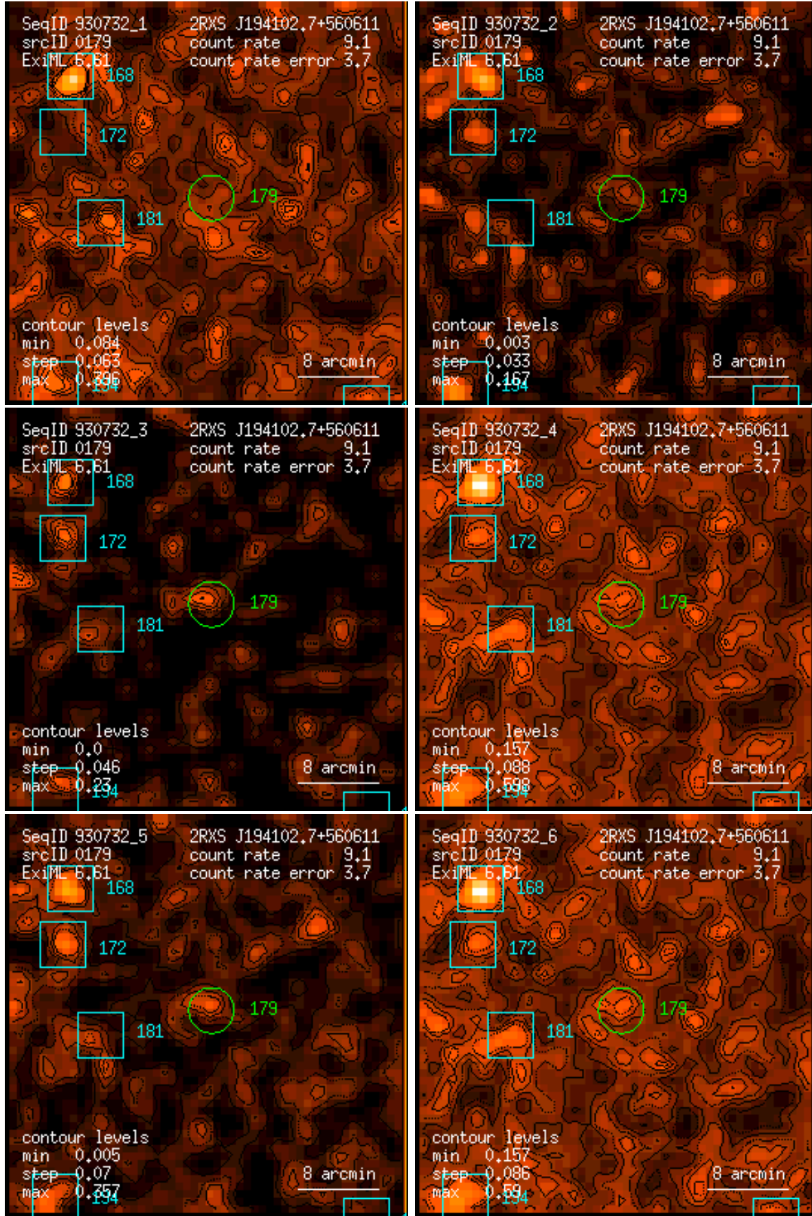
Figure 179: RASS 930732: detection 0179: band rate images, Gaussian filter: (1) PSPC channels 11 – 41, (2) 52 – 90, (3) 91 – 201, (4) 11 – 235, (5) 52 – 201, (6) 11 – 201. Broad band rates in counts/ks. Band rate contour levels in counts/ks/arcmin 2 .
