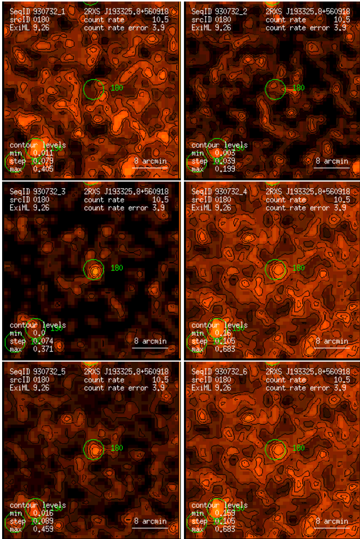
Figure 180: RASS 930732: detection 0180: band rate images, Gaussian filter: (1) PSPC channels 11 – 41, (2) 52 – 90, (3) 91 – 201, (4) 11 – 235, (5) 52 – 201, (6) 11 – 201. Broad band rates in counts/ks. Band rate contour levels in counts/ks/arcmin 2 .
