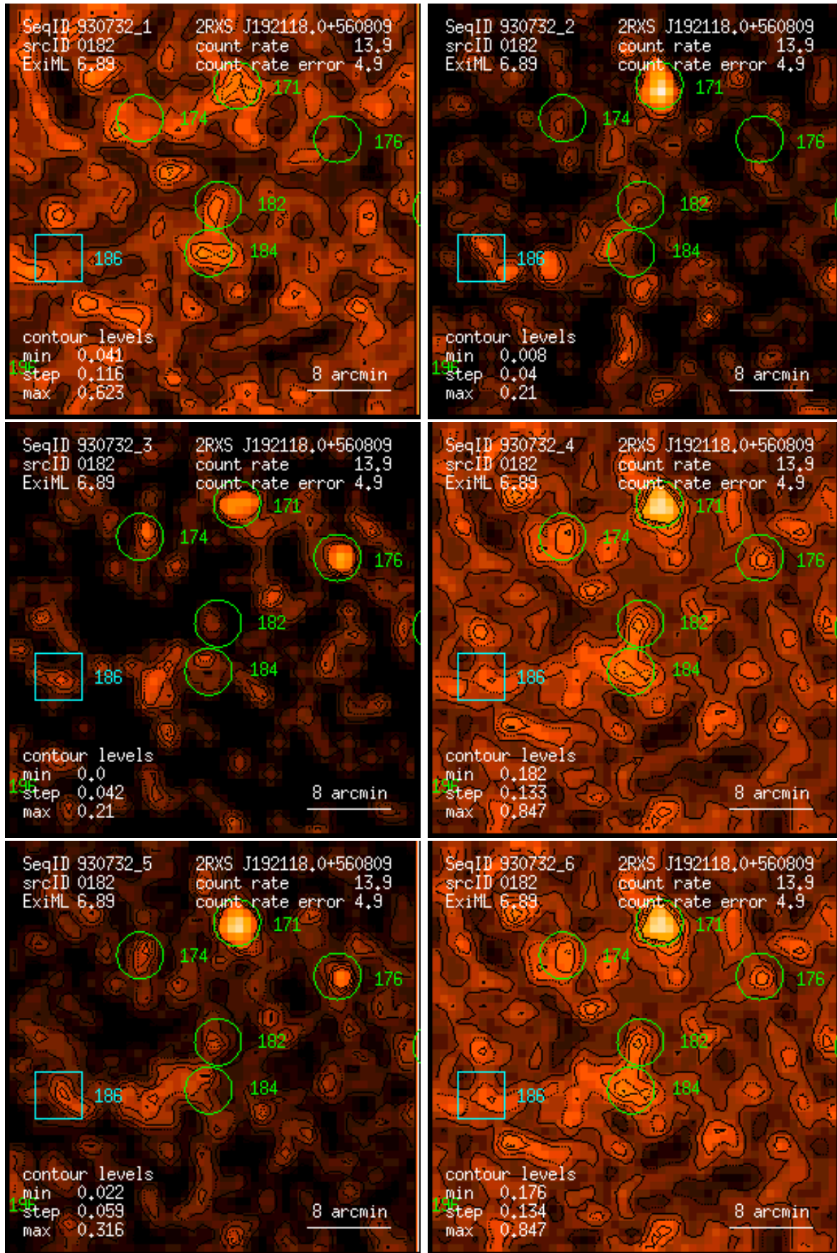
Figure 182: RASS 930732: detection 0182: band rate images, Gaussian filter: (1) PSPC channels 11 – 41, (2) 52 – 90, (3) 91 – 201, (4) 11 – 235, (5) 52 – 201, (6) 11 – 201. Broad band rates in counts/ks. Band rate contour levels in counts/ks/arcmin 2 .
