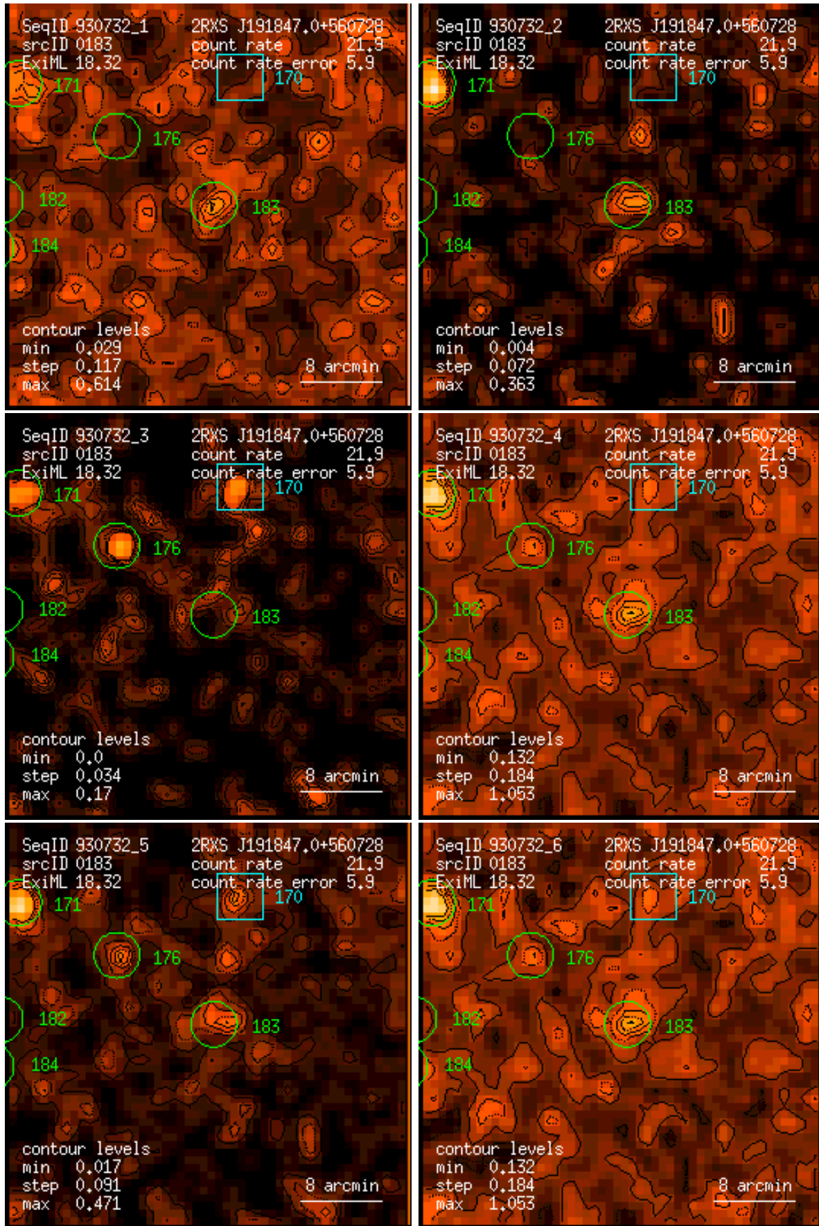
Figure 183: RASS 930732: detection 0183: band rate images, Gaussian filter: (1) PSPC channels 11 – 41, (2) 52 – 90, (3) 91 – 201, (4) 11 – 235, (5) 52 – 201, (6) 11 – 201. Broad band rates in counts/ks. Band rate contour levels in counts/ks/arcmin 2 .
